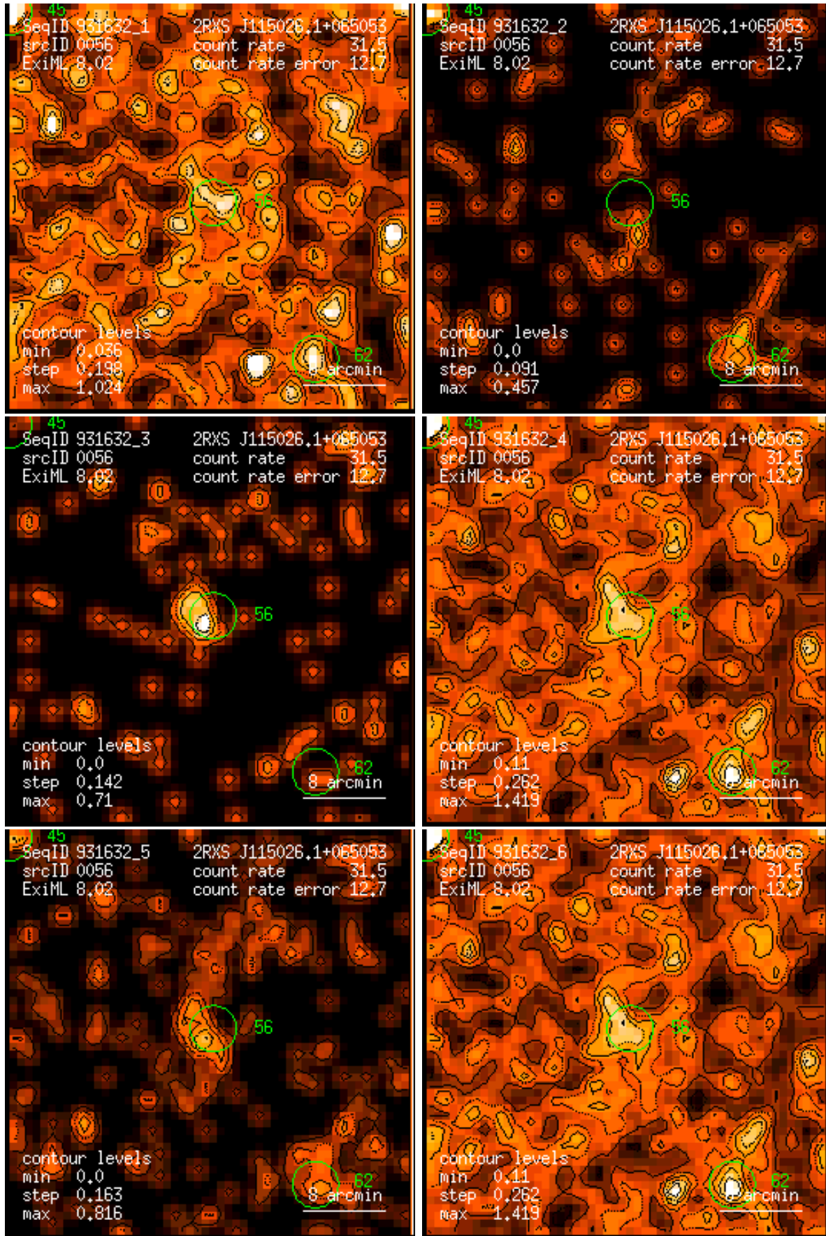
Figure 56: RASS 931632: detection 0056: band rate images, Gaussian filter: (1) PSPC channels 11 – 41, (2) 52 – 90, (3) 91 – 201, (4) 11 – 235, (5) 52 – 201, (6) 11 – 201. Broad band rates in counts/ks. Band rate contour levels in counts/ks/arcmin 2 .
