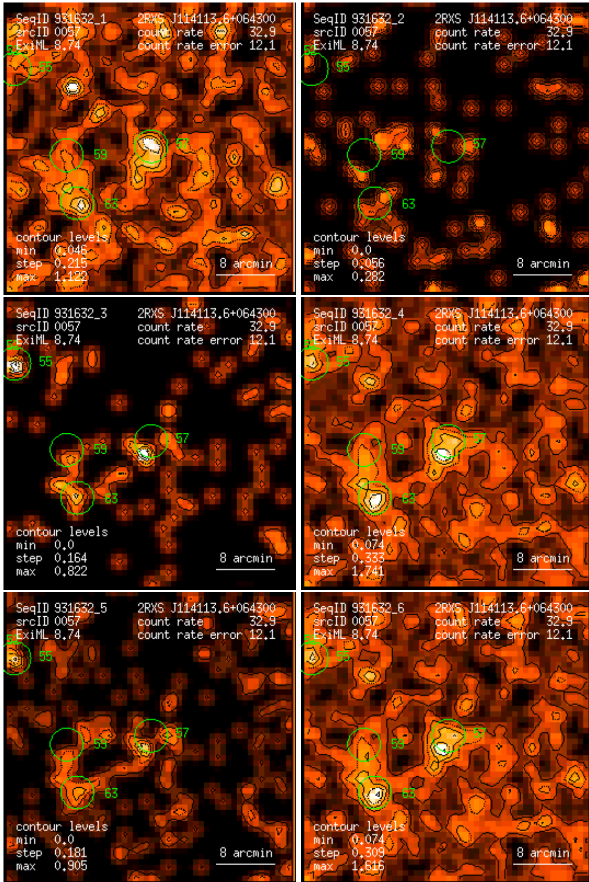
Figure 57: RASS 931632: detection 0057: band rate images, Gaussian filter: (1) PSPC channels 11 – 41, (2) 52 – 90, (3) 91 – 201, (4) 11 – 235, (5) 52 – 201, (6) 11 – 201. Broad band rates in counts/ks. Band rate contour levels in counts/ks/arcmin 2 .
