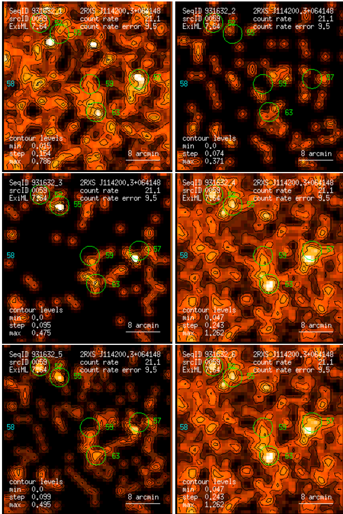
Figure 59: RASS 931632: detection 0059: band rate images, Gaussian filter: (1) PSPC channels 11 – 41, (2) 52 – 90, (3) 91 – 201, (4) 11 – 235, (5) 52 – 201, (6) 11 – 201. Broad band rates in counts/ks. Band rate contour levels in counts/ks/arcmin 2 .
