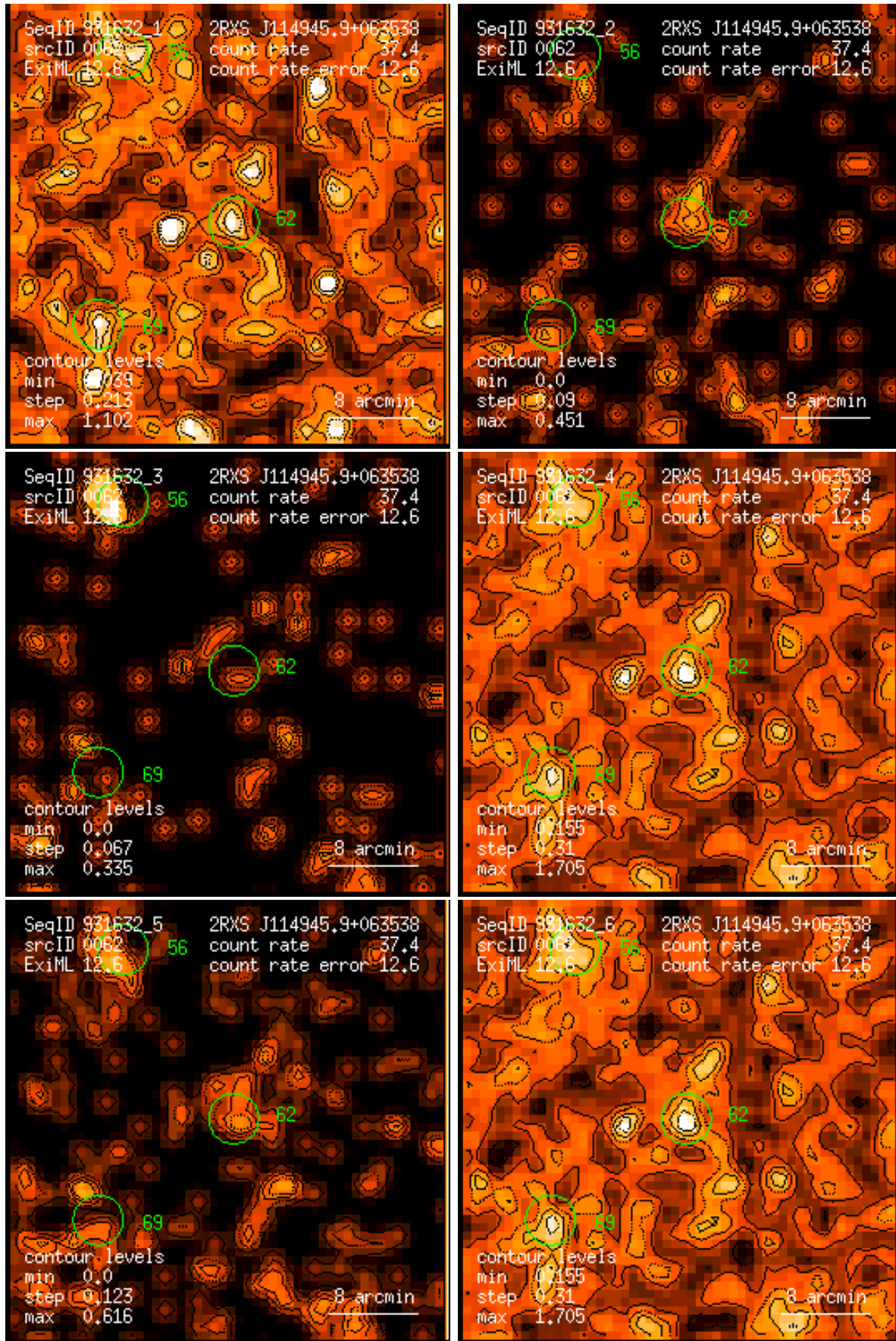
Figure 62: RASS 931632: detection 0062: band rate images, Gaussian filter: (1) PSPC channels 11 – 41, (2) 52 – 90, (3) 91 – 201, (4) 11 – 235, (5) 52 – 201, (6) 11 – 201. Broad band rates in counts/ks. Band rate contour levels in counts/ks/arcmin 2 .
