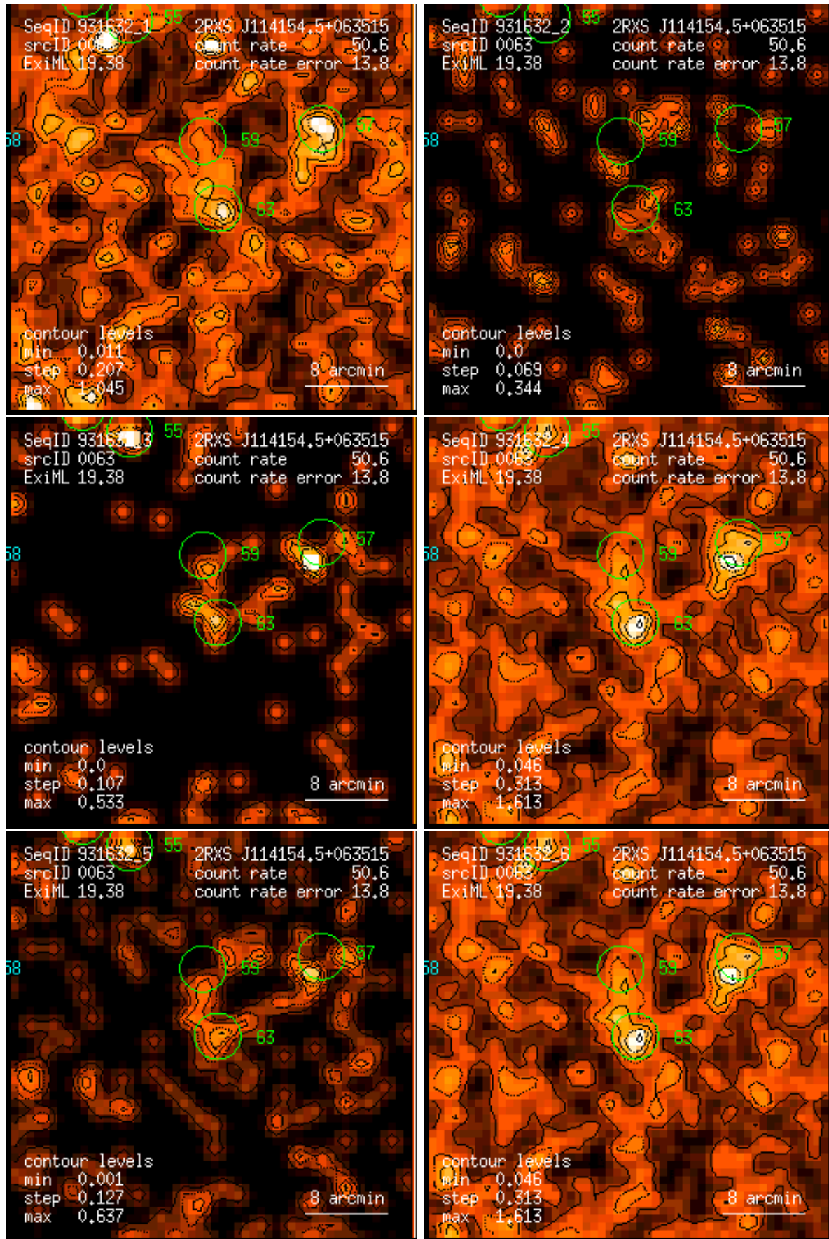
Figure 63: RASS 931632: detection 0063: band rate images, Gaussian filter: (1) PSPC channels 11 – 41, (2) 52 – 90, (3) 91 – 201, (4) 11 – 235, (5) 52 – 201, (6) 11 – 201. Broad band rates in counts/ks. Band rate contour levels in counts/ks/arcmin 2 .
