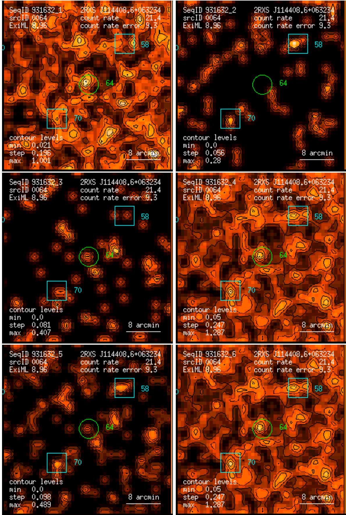
Figure 64: RASS 931632: detection 0064: band rate images, Gaussian filter: (1) PSPC channels 11 – 41, (2) 52 – 90, (3) 91 – 201, (4) 11 – 235, (5) 52 – 201, (6) 11 – 201. Broad band rates in counts/ks. Band rate contour levels in counts/ks/arcmin 2 .
