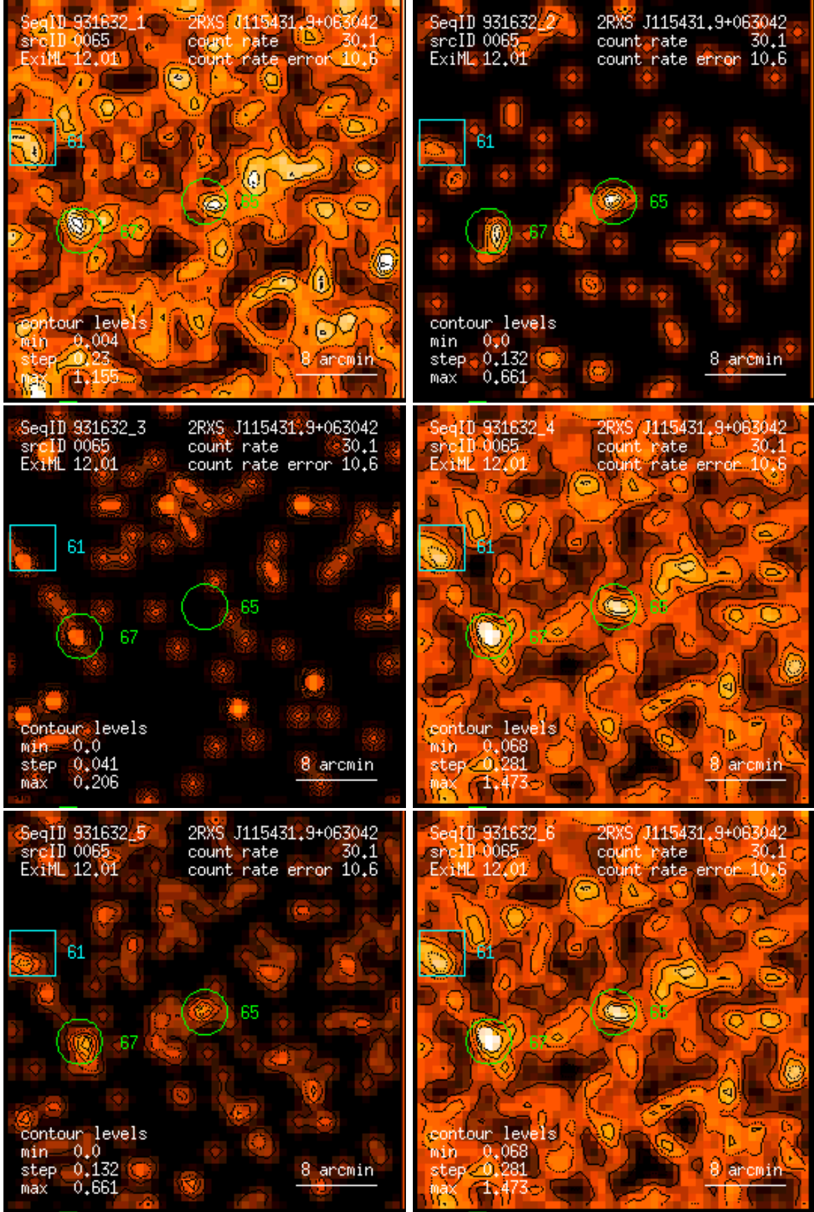
Figure 65: RASS 931632: detection 0065: band rate images, Gaussian filter: (1) PSPC channels 11 – 41, (2) 52 – 90, (3) 91 – 201, (4) 11 – 235, (5) 52 – 201, (6) 11 – 201. Broad band rates in counts/ks. Band rate contour levels in counts/ks/arcmin 2 .
