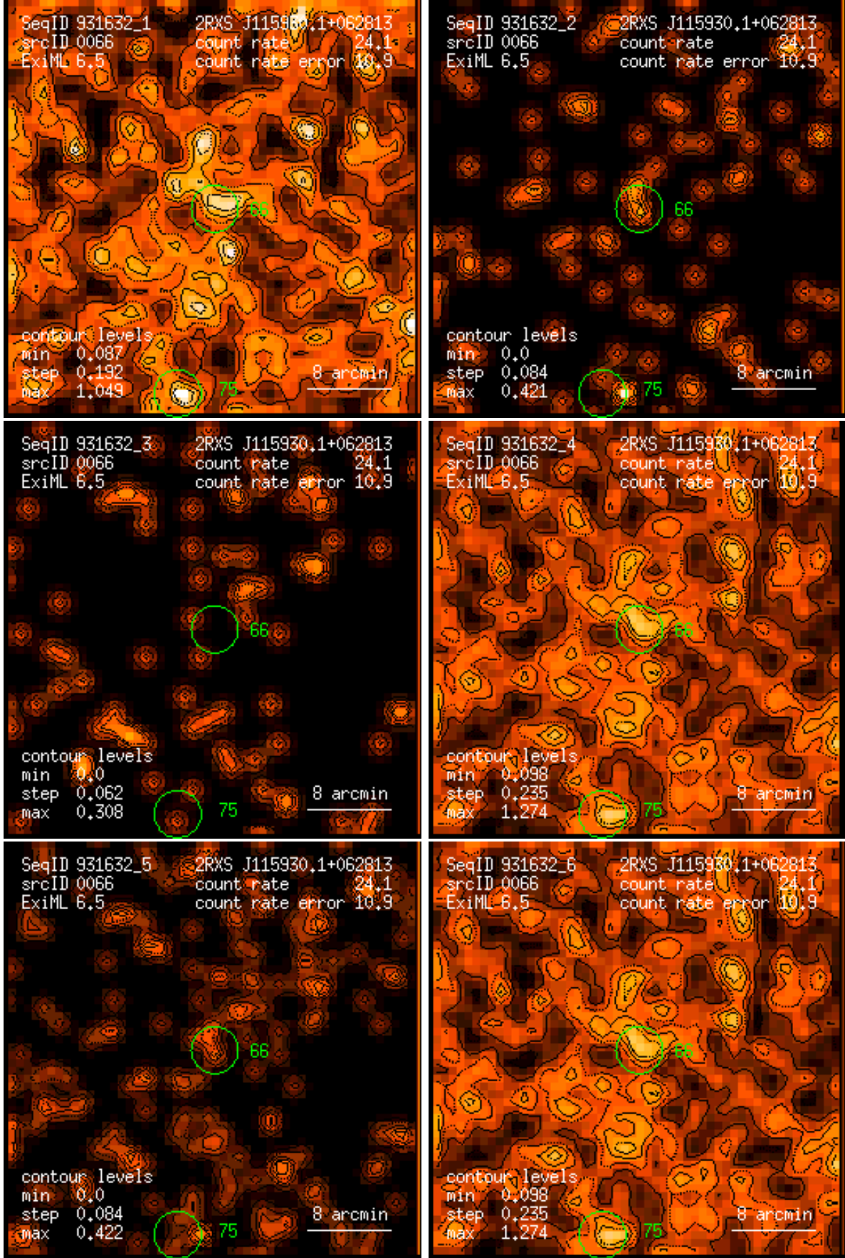
Figure 66: RASS 931632: detection 0066: band rate images, Gaussian filter: (1) PSPC channels 11 – 41, (2) 52 – 90, (3) 91 – 201, (4) 11 – 235, (5) 52 – 201, (6) 11 – 201. Broad band rates in counts/ks. Band rate contour levels in counts/ks/arcmin 2 .
