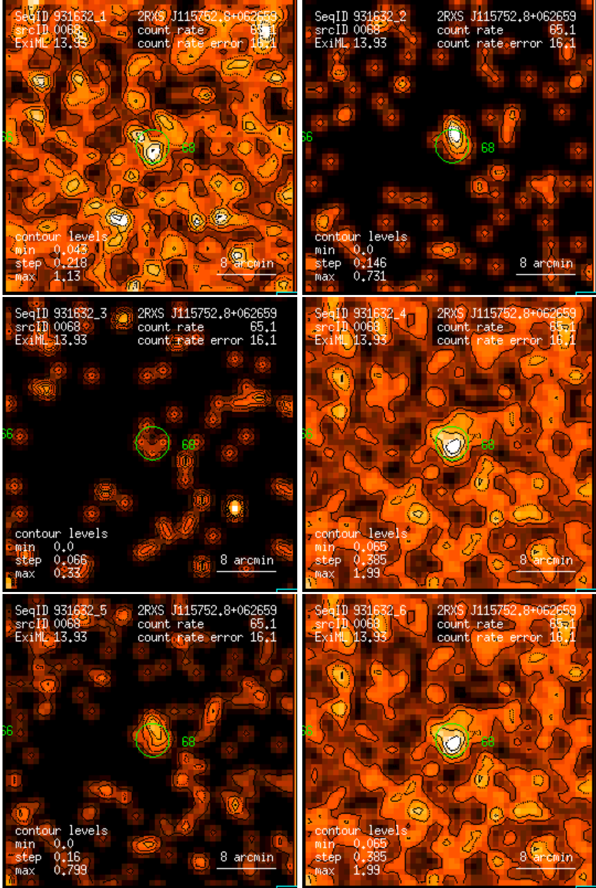
Figure 68: RASS 931632: detection 0068: band rate images, Gaussian filter: (1) PSPC channels 11 – 41, (2) 52 – 90, (3) 91 – 201, (4) 11 – 235, (5) 52 – 201, (6) 11 – 201. Broad band rates in counts/ks. Band rate contour levels in counts/ks/arcmin 2 .
