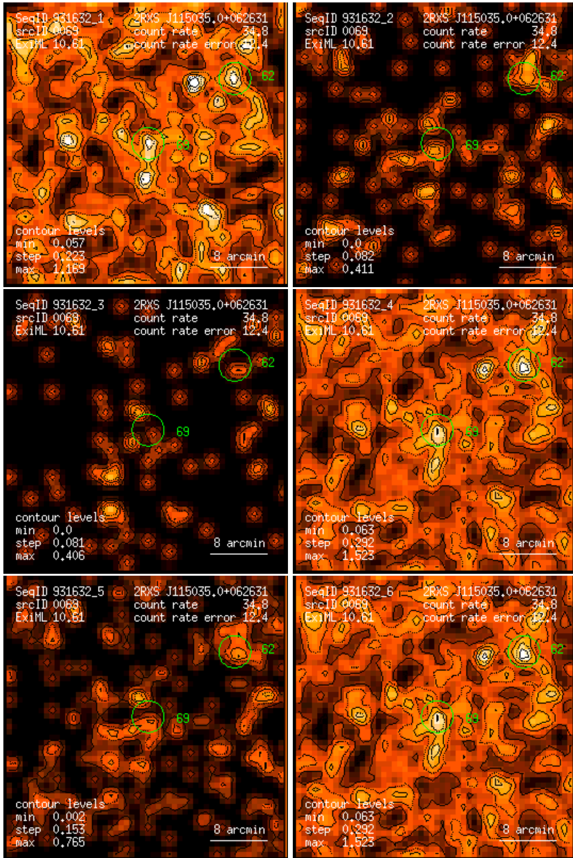
Figure 69: RASS 931632: detection 0069: band rate images, Gaussian filter: (1) PSPC channels 11 – 41, (2) 52 – 90, (3) 91 – 201, (4) 11 – 235, (5) 52 – 201, (6) 11 – 201. Broad band rates in counts/ks. Band rate contour levels in counts/ks/arcmin 2 .
