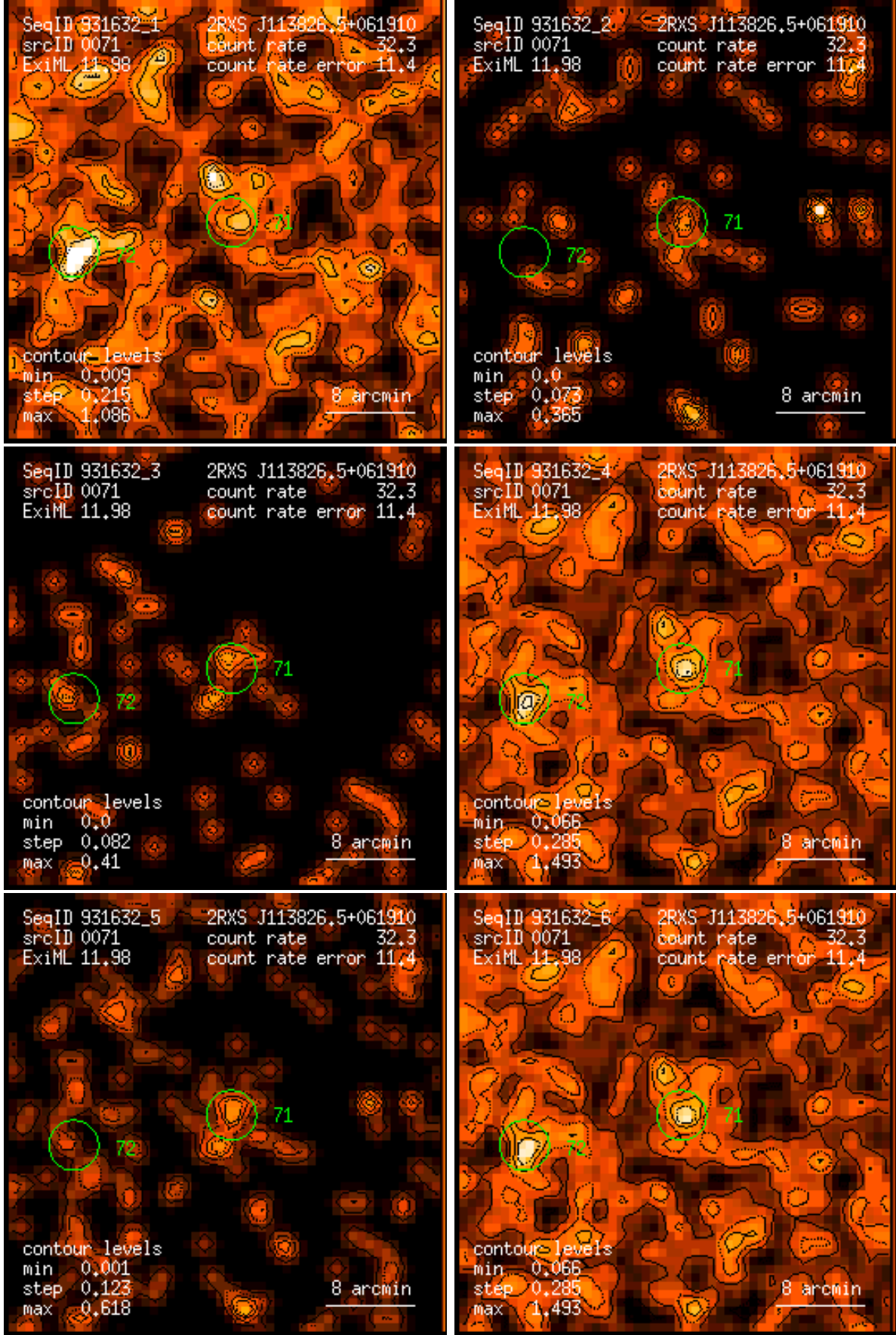
Figure 71: RASS 931632: detection 0071: band rate images, Gaussian filter: (1) PSPC channels 11 – 41, (2) 52 – 90, (3) 91 – 201, (4) 11 – 235, (5) 52 – 201, (6) 11 – 201. Broad band rates in counts/ks. Band rate contour levels in counts/ks/arcmin 2 .
