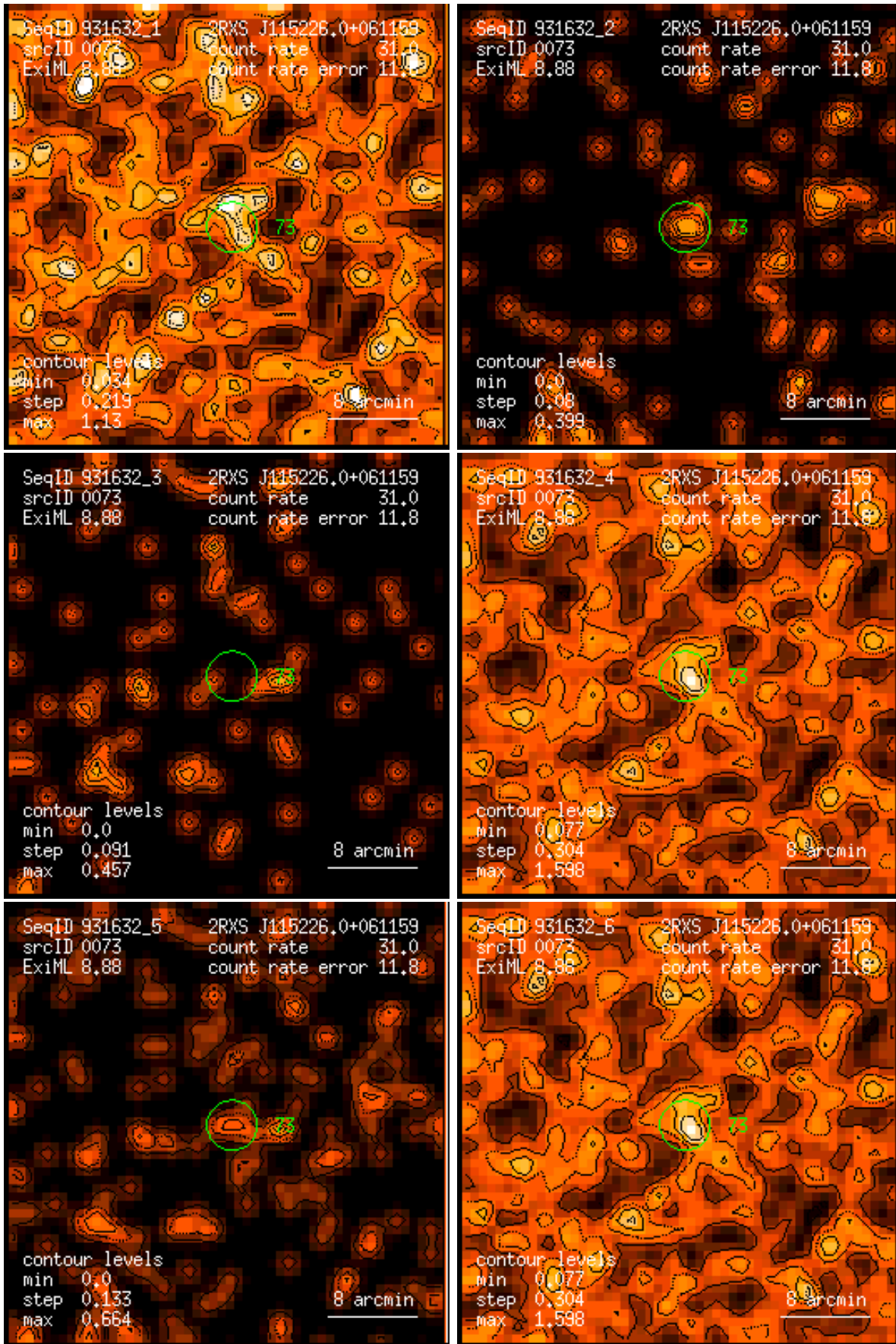
Figure 73: RASS 931632: detection 0073: band rate images, Gaussian filter: (1) PSPC channels 11 – 41, (2) 52 – 90, (3) 91 – 201, (4) 11 – 235, (5) 52 – 201, (6) 11 – 201. Broad band rates in counts/ks. Band rate contour levels in counts/ks/arcmin 2 .
