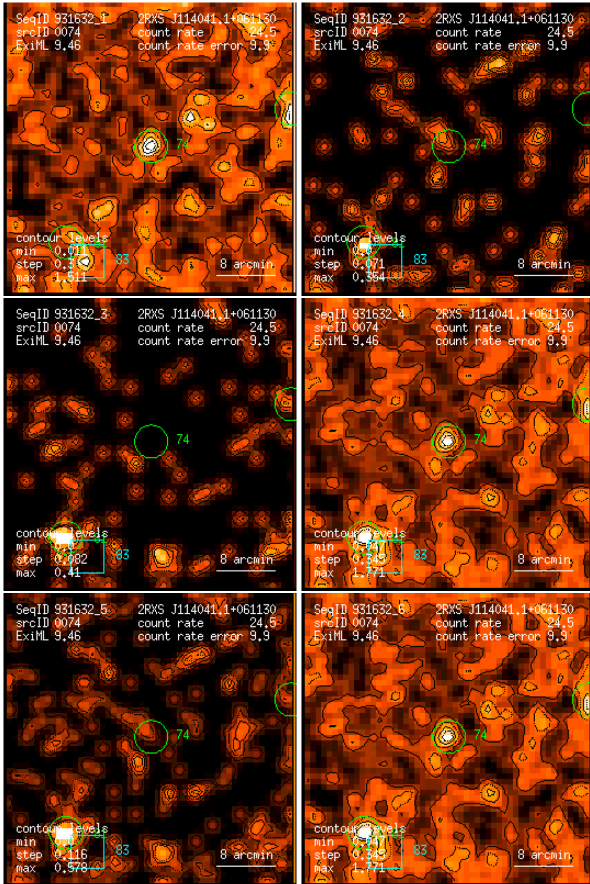
Figure 74: RASS 931632: detection 0074: band rate images, Gaussian filter: (1) PSPC channels 11 – 41, (2) 52 – 90, (3) 91 – 201, (4) 11 – 235, (5) 52 – 201, (6) 11 – 201. Broad band rates in counts/ks. Band rate contour levels in counts/ks/arcmin 2 .
