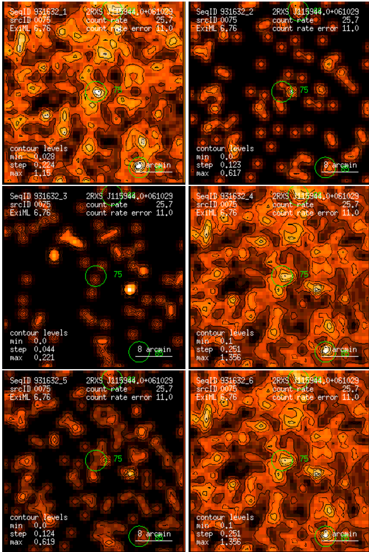
Figure 75: RASS 931632: detection 0075: band rate images, Gaussian filter: (1) PSPC channels 11 – 41, (2) 52 – 90, (3) 91 – 201, (4) 11 – 235, (5) 52 – 201, (6) 11 – 201. Broad band rates in counts/ks. Band rate contour levels in counts/ks/arcmin 2 .
