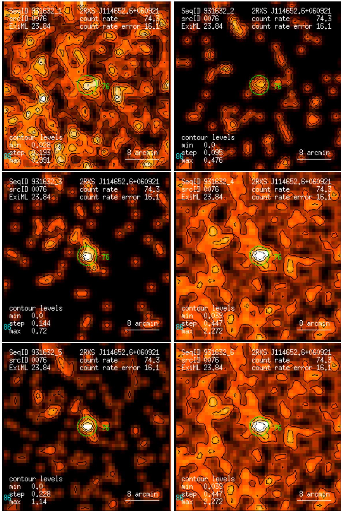
Figure 76: RASS 931632: detection 0076: band rate images, Gaussian filter: (1) PSPC channels 11 – 41, (2) 52 – 90, (3) 91 – 201, (4) 11 – 235, (5) 52 – 201, (6) 11 – 201. Broad band rates in counts/ks. Band rate contour levels in counts/ks/arcmin 2 .
