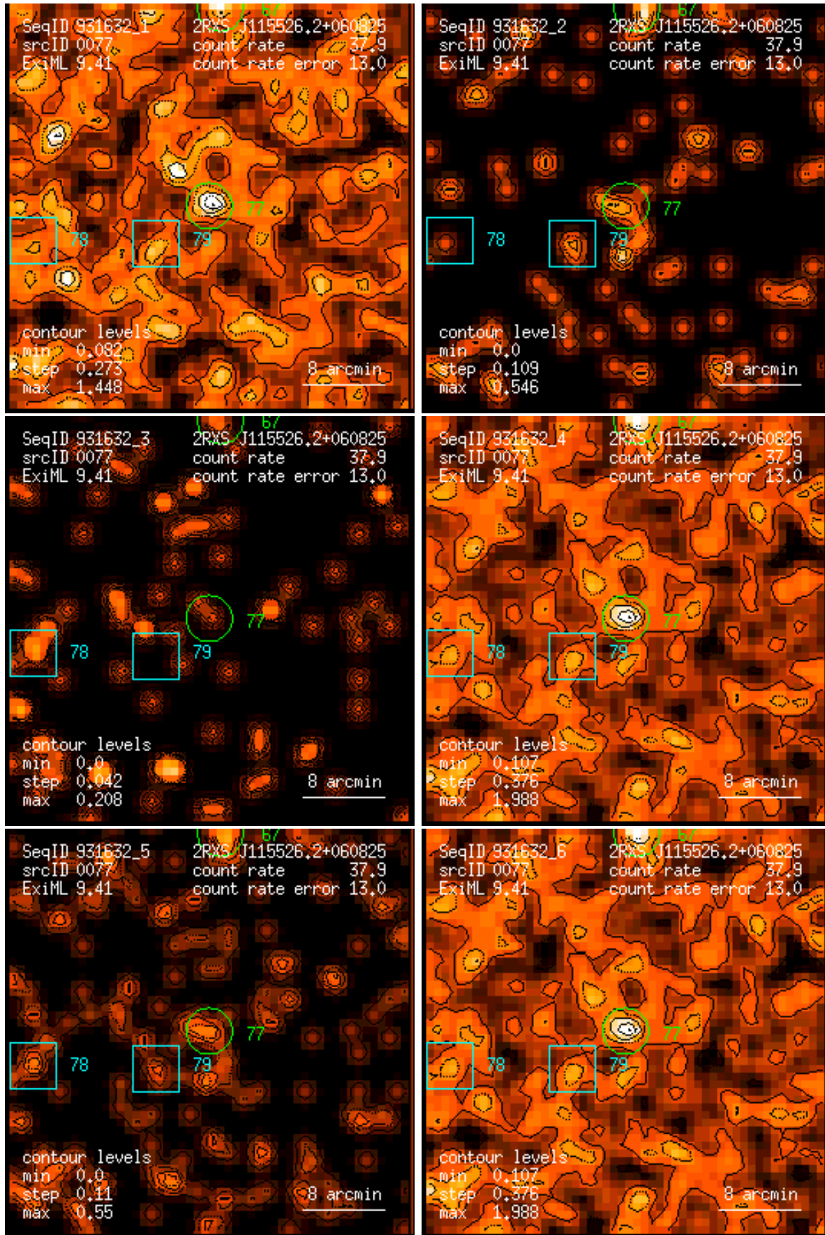
Figure 77: RASS 931632: detection 0077: band rate images, Gaussian filter: (1) PSPC channels 11 – 41, (2) 52 – 90, (3) 91 – 201, (4) 11 – 235, (5) 52 – 201, (6) 11 – 201. Broad band rates in counts/ks. Band rate contour levels in counts/ks/arcmin 2 .
