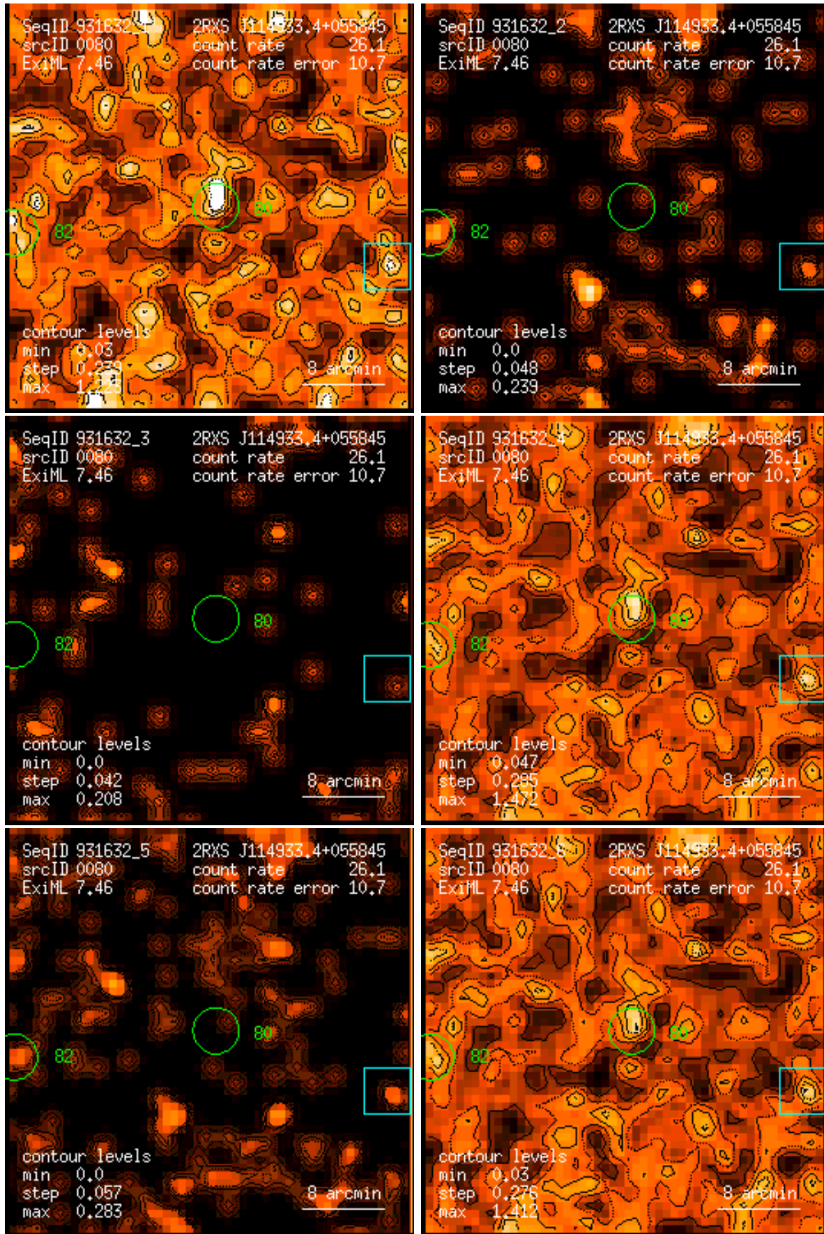
Figure 80: RASS 931632: detection 0080: band rate images, Gaussian filter: (1) PSPC channels 11 – 41, (2) 52 – 90, (3) 91 – 201, (4) 11 – 235, (5) 52 – 201, (6) 11 – 201. Broad band rates in counts/ks. Band rate contour levels in counts/ks/arcmin 2 .
