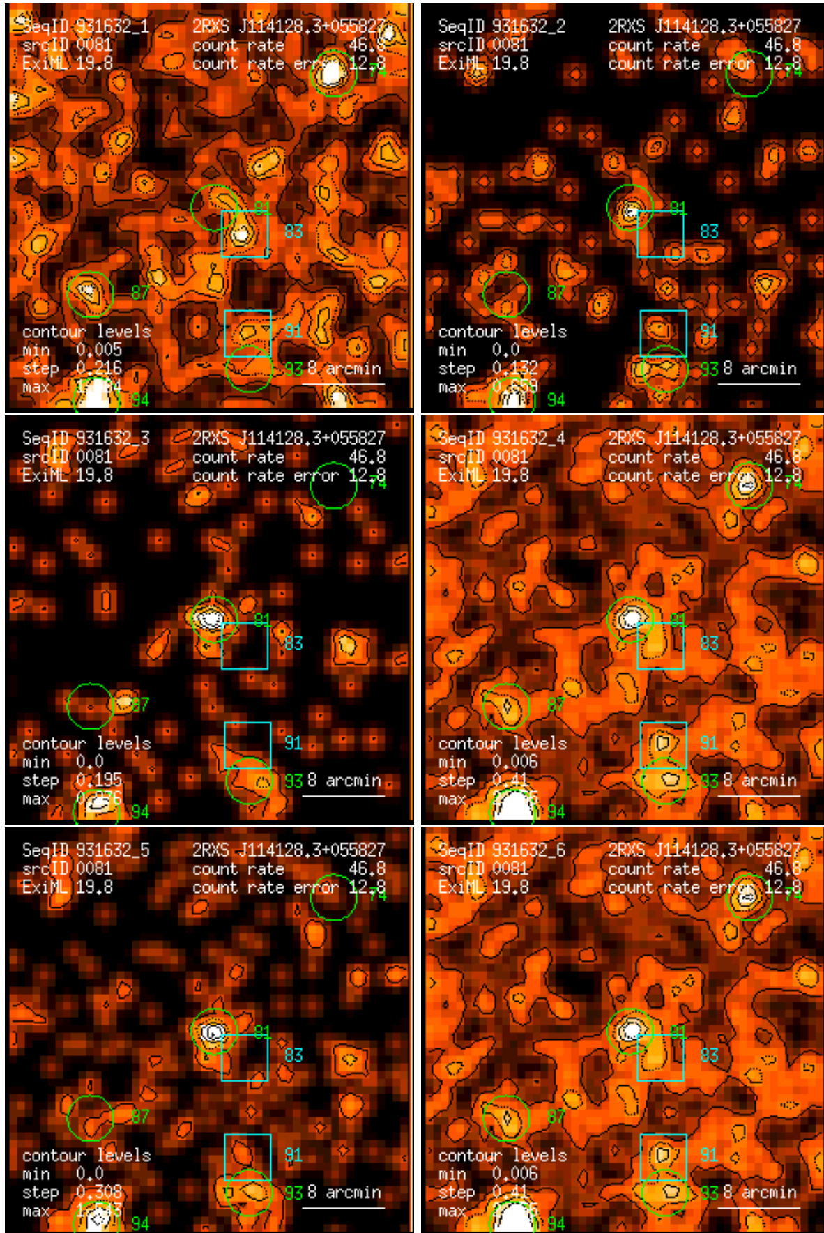
Figure 81: RASS 931632: detection 0081: band rate images, Gaussian filter: (1) PSPC channels 11 – 41, (2) 52 – 90, (3) 91 – 201, (4) 11 – 235, (5) 52 – 201, (6) 11 – 201. Broad band rates in counts/ks. Band rate contour levels in counts/ks/arcmin 2 .
