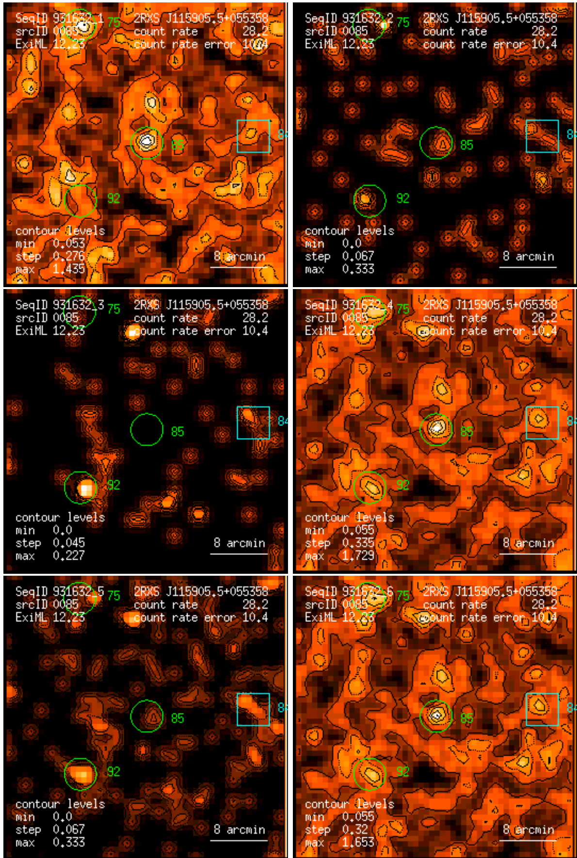
Figure 85: RASS 931632: detection 0085: band rate images, Gaussian filter: (1) PSPC channels 11 – 41, (2) 52 – 90, (3) 91 – 201, (4) 11 – 235, (5) 52 – 201, (6) 11 – 201. Broad band rates in counts/ks. Band rate contour levels in counts/ks/arcmin 2 .
