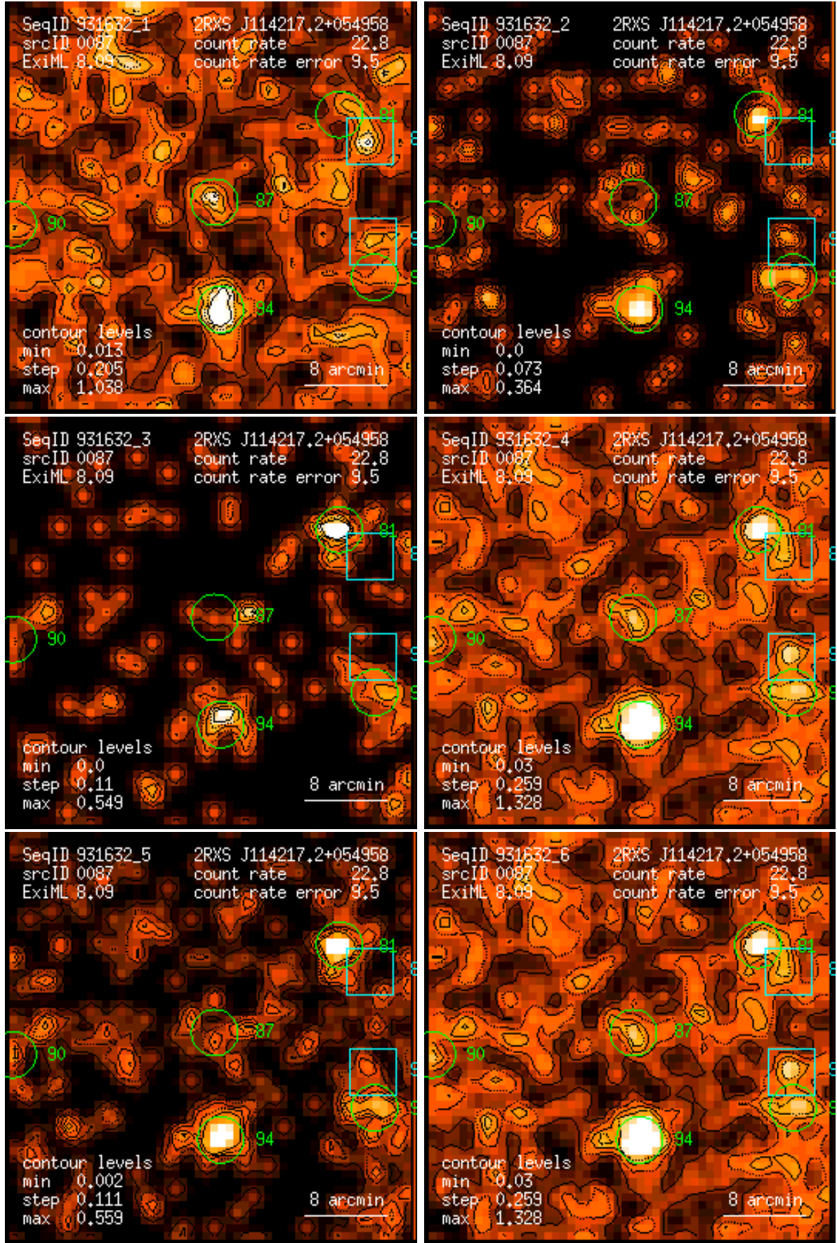
Figure 87: RASS 931632: detection 0087: band rate images, Gaussian filter: (1) PSPC channels 11 – 41, (2) 52 – 90, (3) 91 – 201, (4) 11 – 235, (5) 52 – 201, (6) 11 – 201. Broad band rates in counts/ks. Band rate contour levels in counts/ks/arcmin 2 .
