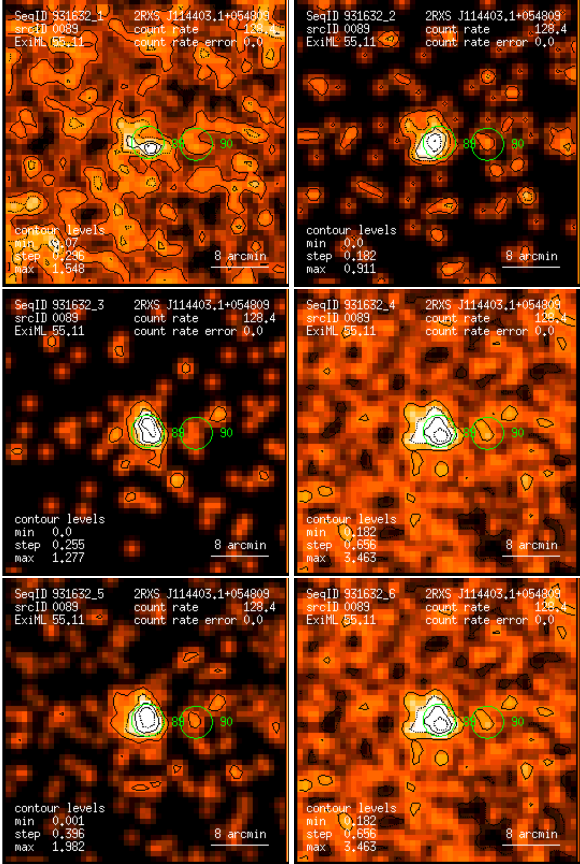
Figure 89: RASS 931632: detection 0089: band rate images, Gaussian filter: (1) PSPC channels 11 – 41, (2) 52 – 90, (3) 91 – 201, (4) 11 – 235, (5) 52 – 201, (6) 11 – 201. Broad band rates in counts/ks. Band rate contour levels in counts/ks/arcmin 2 .
