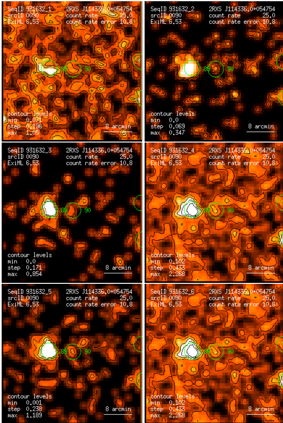
Figure 90: RASS 931632: detection 0090: band rate images, Gaussian filter: (1) PSPC channels 11 – 41, (2) 52 – 90, (3) 91 – 201, (4) 11 – 235, (5) 52 – 201, (6) 11 – 201. Broad band rates in counts/ks. Band rate contour levels in counts/ks/arcmin 2 .
