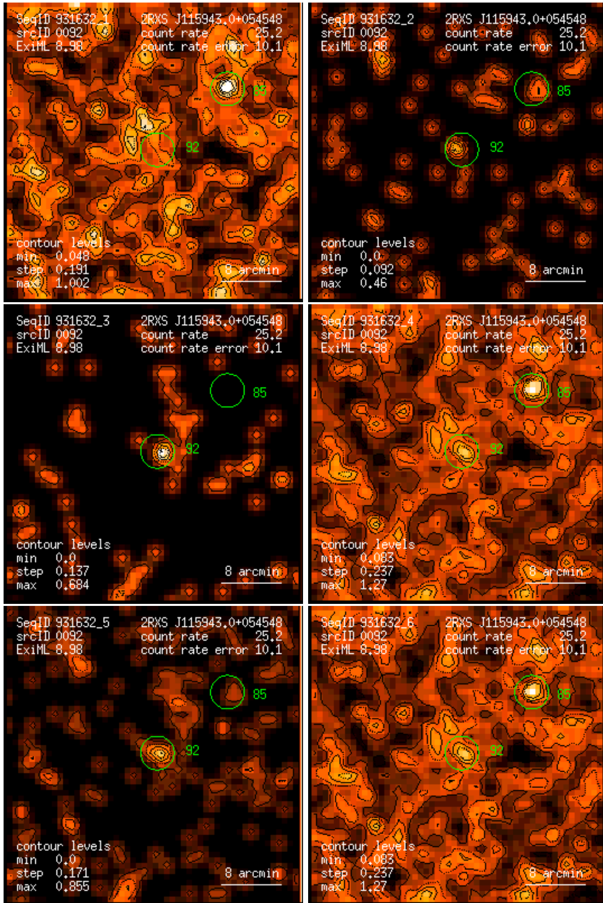
Figure 92: RASS 931632: detection 0092: band rate images, Gaussian filter: (1) PSPC channels 11 – 41, (2) 52 – 90, (3) 91 – 201, (4) 11 – 235, (5) 52 – 201, (6) 11 – 201. Broad band rates in counts/ks. Band rate contour levels in counts/ks/arcmin 2 .
