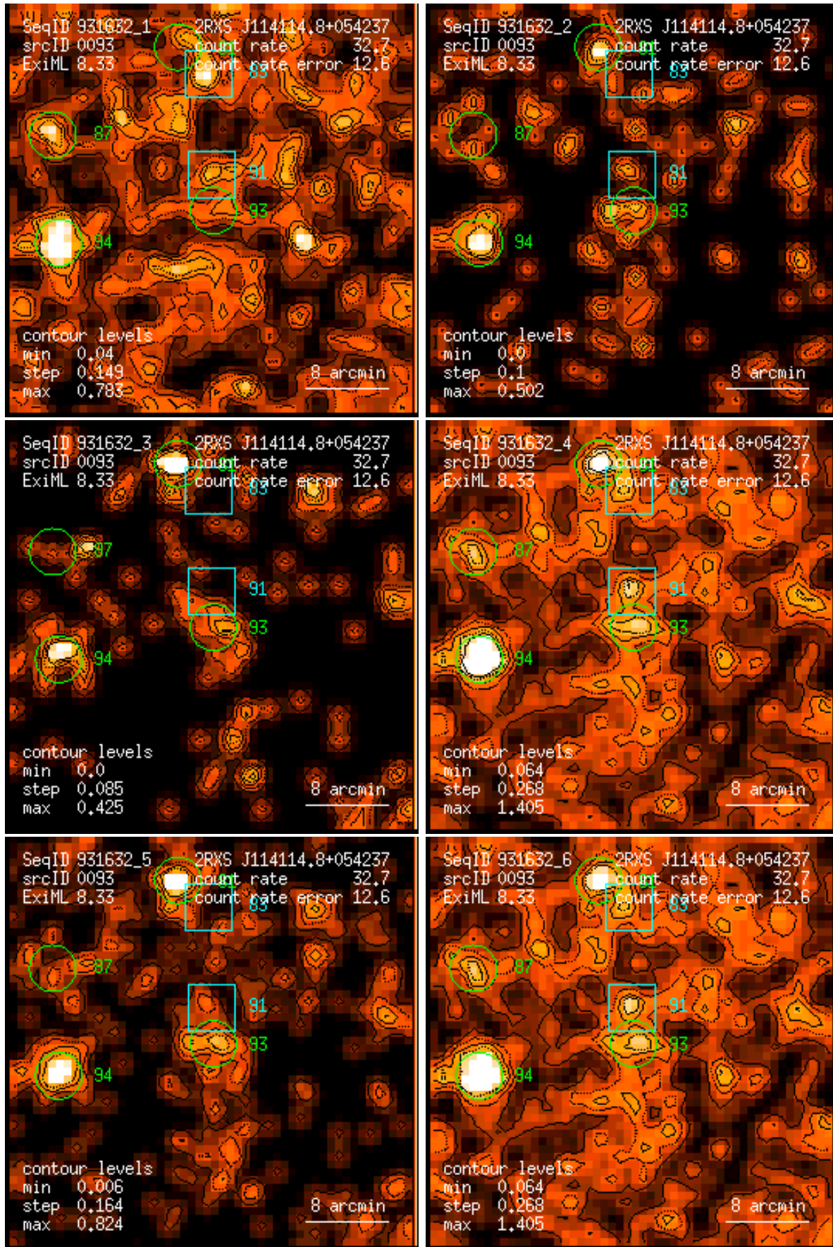
Figure 93: RASS 931632: detection 0093: band rate images, Gaussian filter: (1) PSPC channels 11 – 41, (2) 52 – 90, (3) 91 – 201, (4) 11 – 235, (5) 52 – 201, (6) 11 – 201. Broad band rates in counts/ks. Band rate contour levels in counts/ks/arcmin 2 .
