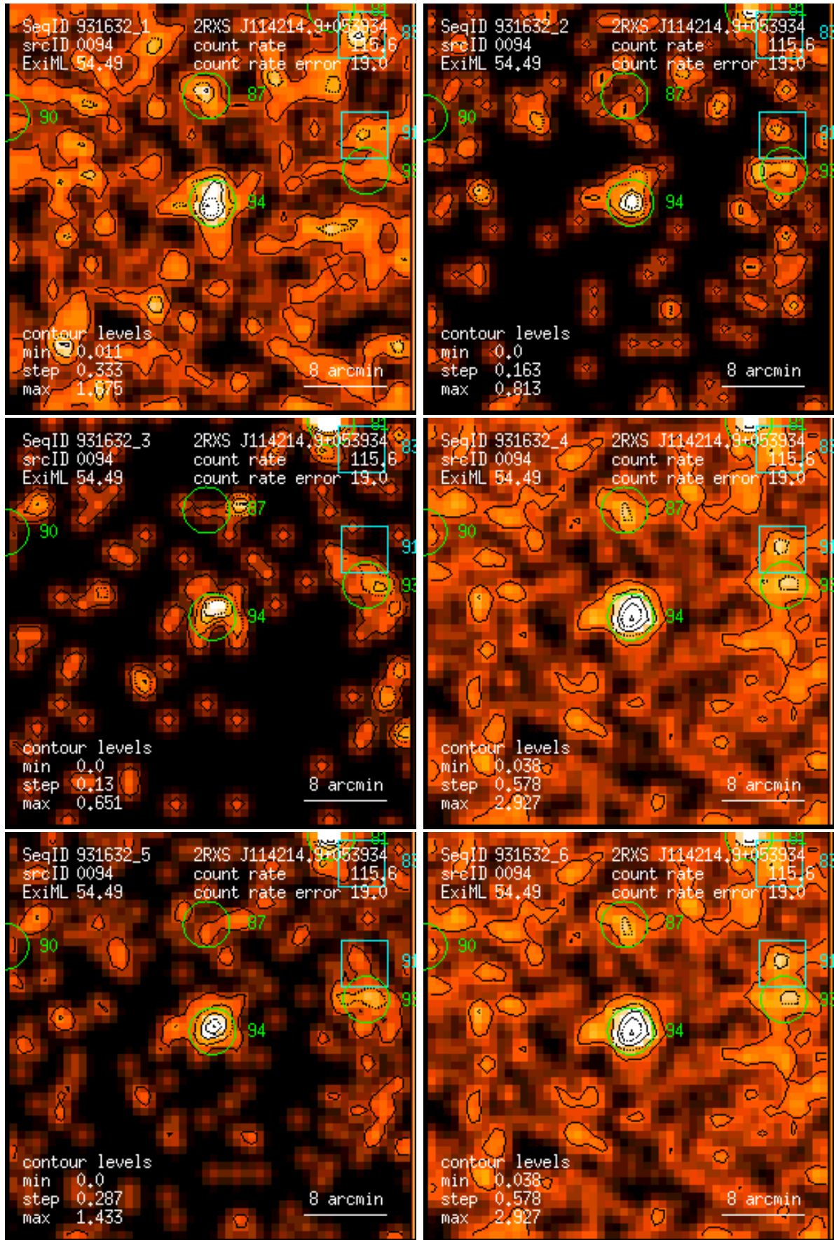
Figure 94: RASS 931632: detection 0094: band rate images, Gaussian filter: (1) PSPC channels 11 – 41, (2) 52 – 90, (3) 91 – 201, (4) 11 – 235, (5) 52 – 201, (6) 11 – 201. Broad band rates in counts/ks. Band rate contour levels in counts/ks/arcmin 2 .
