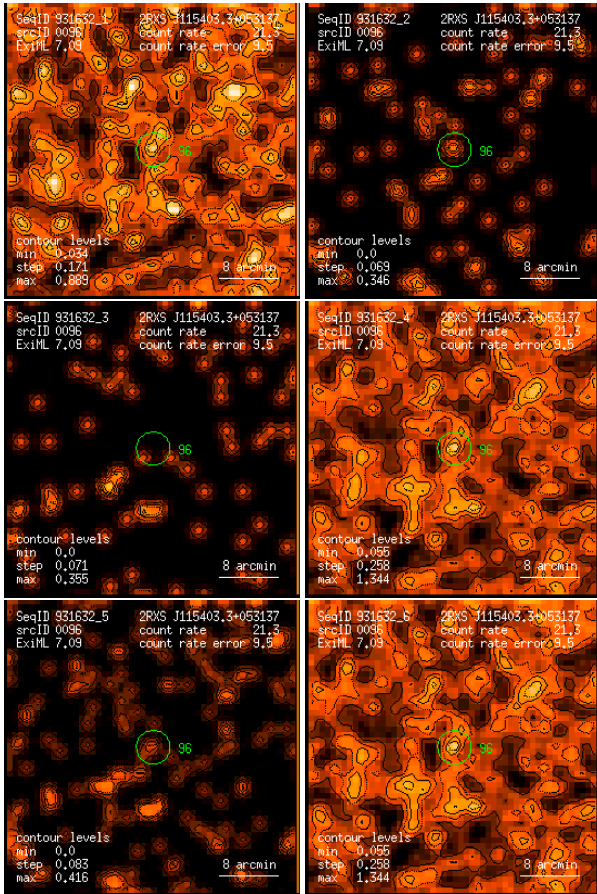
Figure 96: RASS 931632: detection 0096: band rate images, Gaussian filter: (1) PSPC channels 11 – 41, (2) 52 – 90, (3) 91 – 201, (4) 11 – 235, (5) 52 – 201, (6) 11 – 201. Broad band rates in counts/ks. Band rate contour levels in counts/ks/arcmin 2 .
