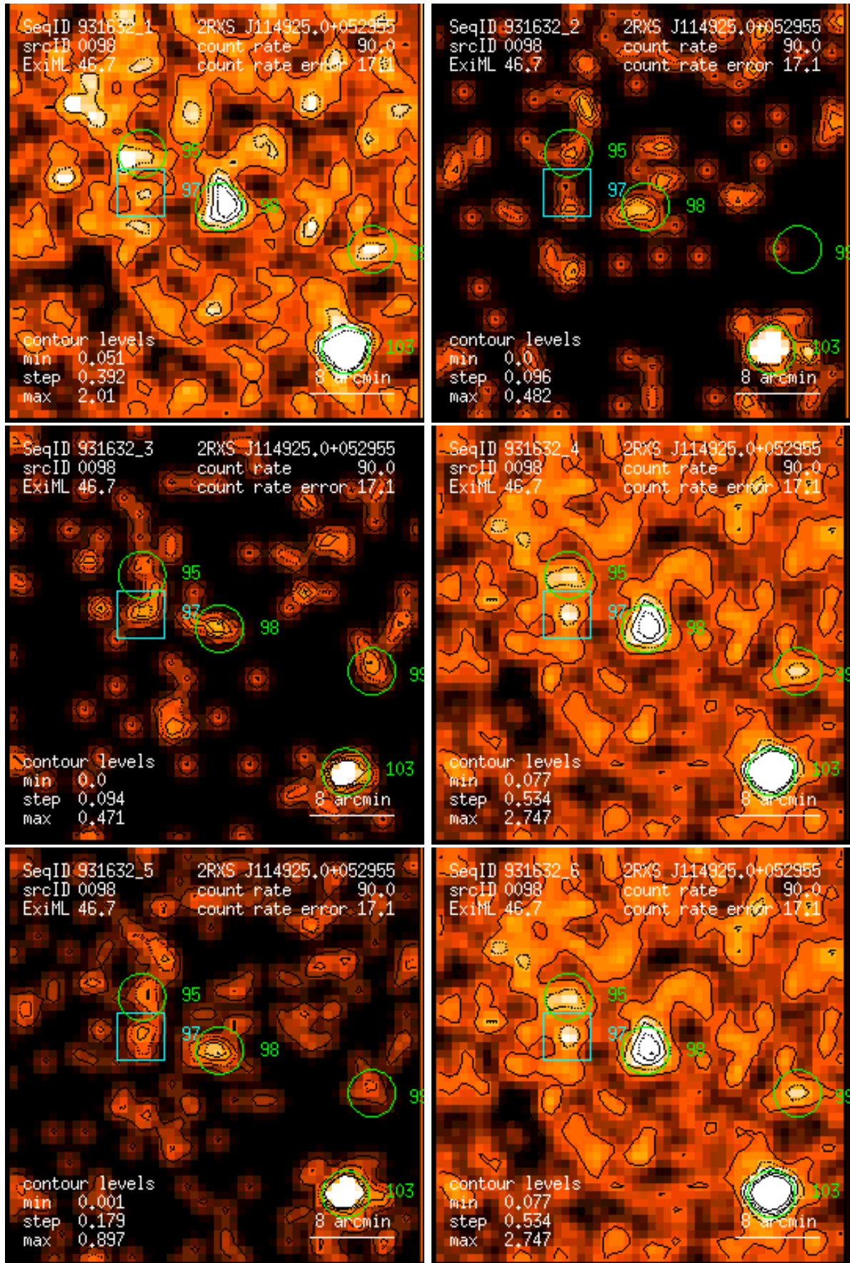
Figure 98: RASS 931632: detection 0098: band rate images, Gaussian filter: (1) PSPC channels 11 – 41, (2) 52 – 90, (3) 91 – 201, (4) 11 – 235, (5) 52 – 201, (6) 11 – 201. Broad band rates in counts/ks. Band rate contour levels in counts/ks/arcmin 2 .
