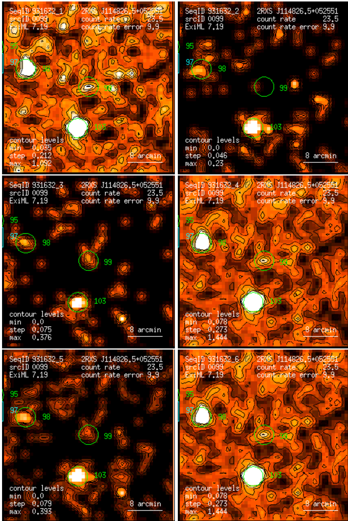
Figure 99: RASS 931632: detection 0099: band rate images, Gaussian filter: (1) PSPC channels 11 – 41, (2) 52 – 90, (3) 91 – 201, (4) 11 – 235, (5) 52 – 201, (6) 11 – 201. Broad band rates in counts/ks. Band rate contour levels in counts/ks/arcmin 2 .
