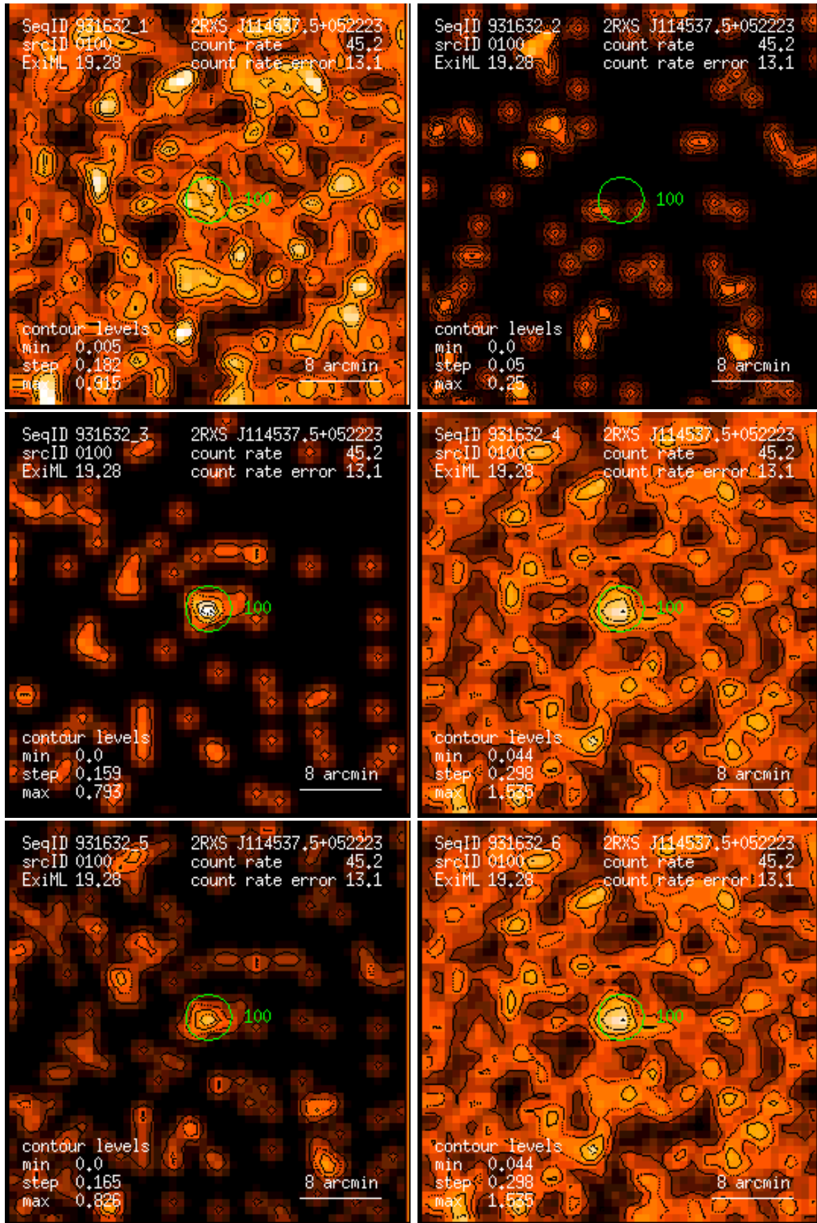
Figure 100: RASS 931632: detection 0100: band rate images, Gaussian filter: (1) PSPC channels 11 – 41, (2) 52 – 90, (3) 91 – 201, (4) 11 – 235, (5) 52 – 201, (6) 11 – 201. Broad band rates in counts/ks. Band rate contour levels in counts/ks/arcmin 2 .
