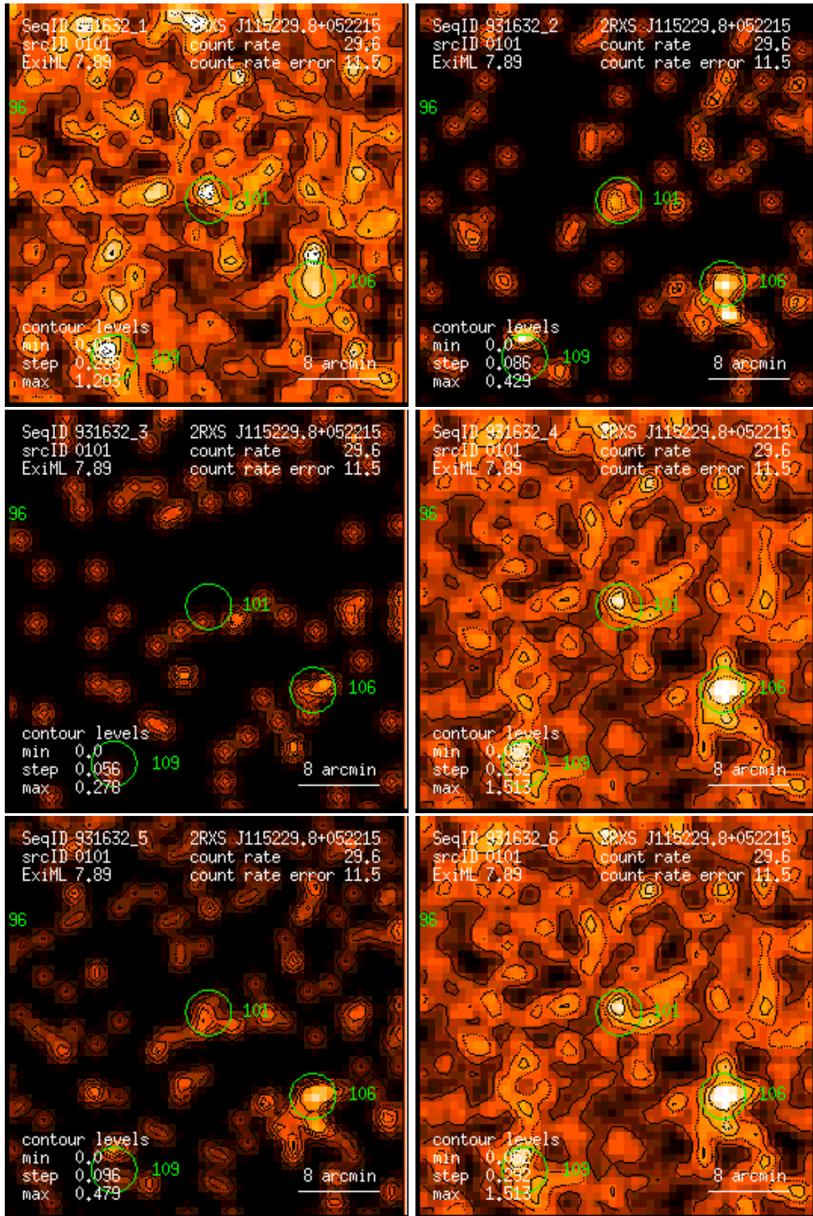
Figure 101: RASS 931632: detection 0101: band rate images, Gaussian filter: (1) PSPC channels 11 – 41, (2) 52 – 90, (3) 91 – 201, (4) 11 – 235, (5) 52 – 201, (6) 11 – 201. Broad band rates in counts/ks. Band rate contour levels in counts/ks/arcmin 2 .
