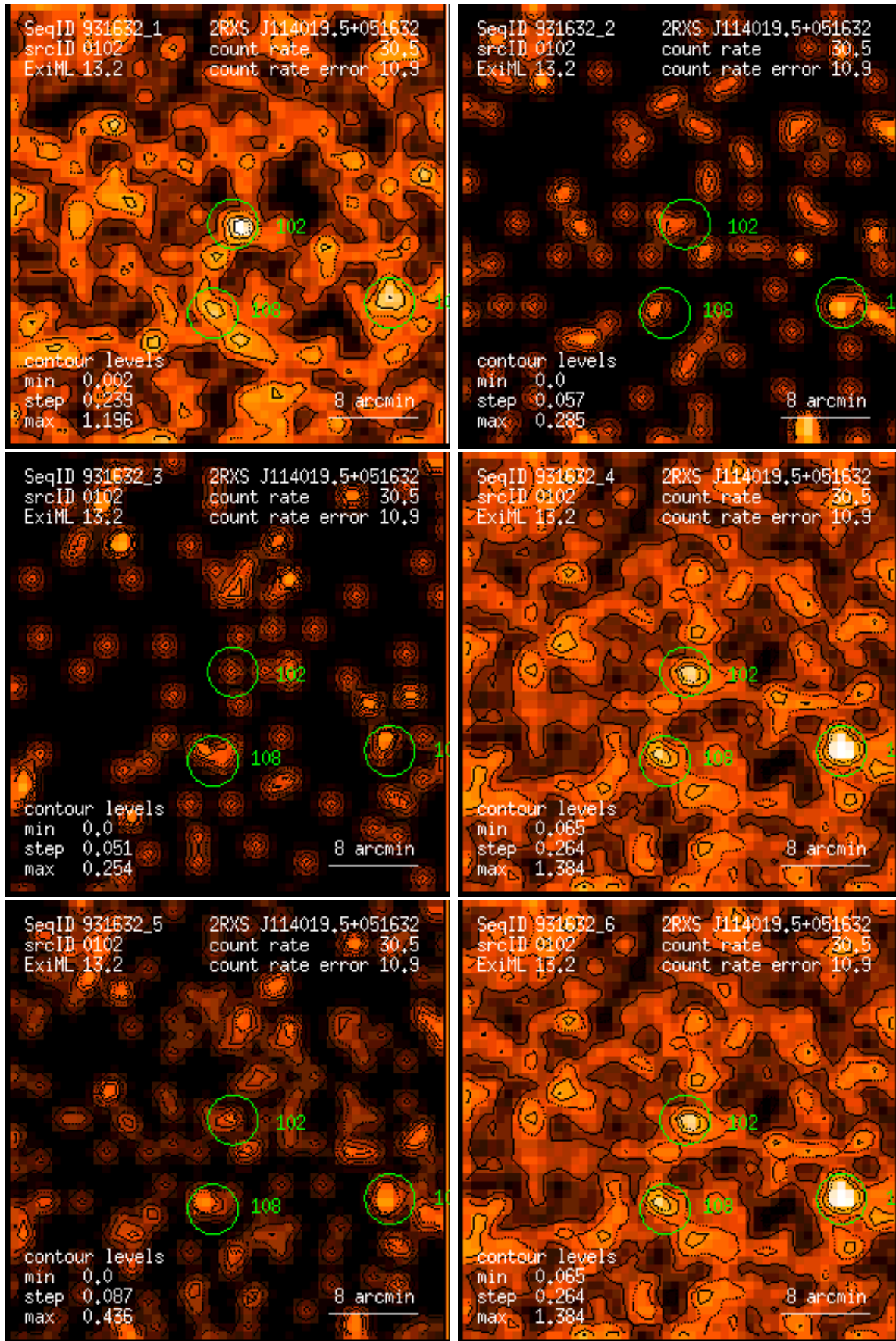
Figure 102: RASS 931632: detection 0102: band rate images, Gaussian filter: (1) PSPC channels 11 – 41, (2) 52 – 90, (3) 91 – 201, (4) 11 – 235, (5) 52 – 201, (6) 11 – 201. Broad band rates in counts/ks. Band rate contour levels in counts/ks/arcmin 2 .
