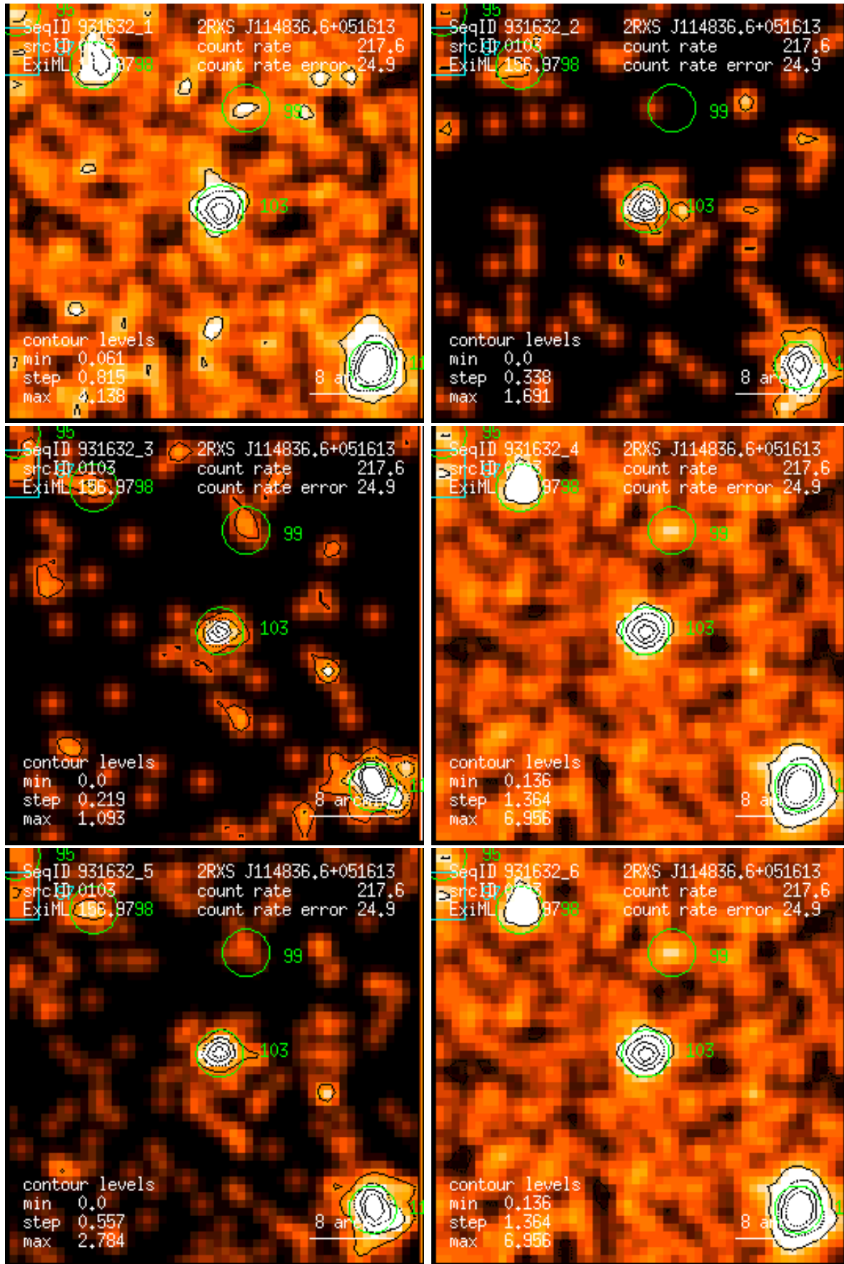
Figure 103: RASS 931632: detection 0103: band rate images, Gaussian filter: (1) PSPC channels 11 – 41, (2) 52 – 90, (3) 91 – 201, (4) 11 – 235, (5) 52 – 201, (6) 11 – 201. Broad band rates in counts/ks. Band rate contour levels in counts/ks/arcmin 2 .
