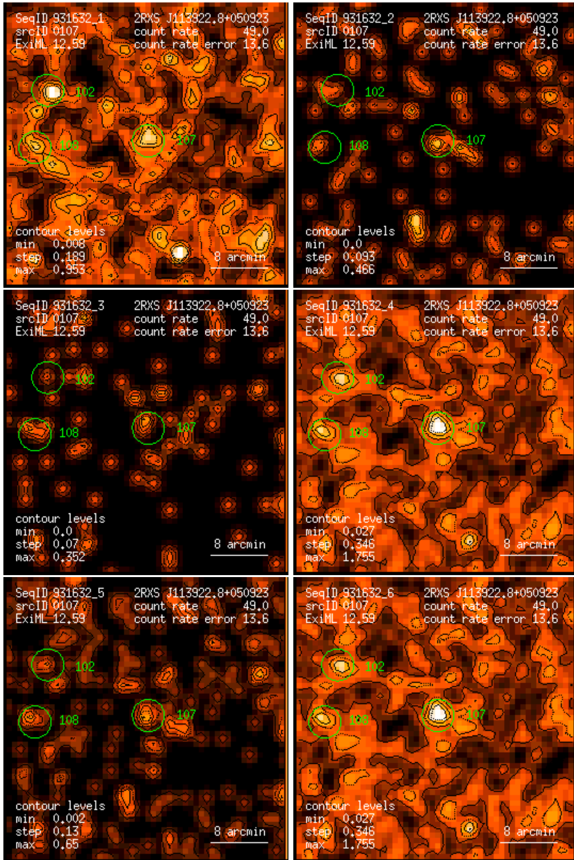
Figure 107: RASS 931632: detection 0107: band rate images, Gaussian filter: (1) PSPC channels 11 – 41, (2) 52 – 90, (3) 91 – 201, (4) 11 – 235, (5) 52 – 201, (6) 11 – 201. Broad band rates in counts/ks. Band rate contour levels in counts/ks/arcmin 2 .
