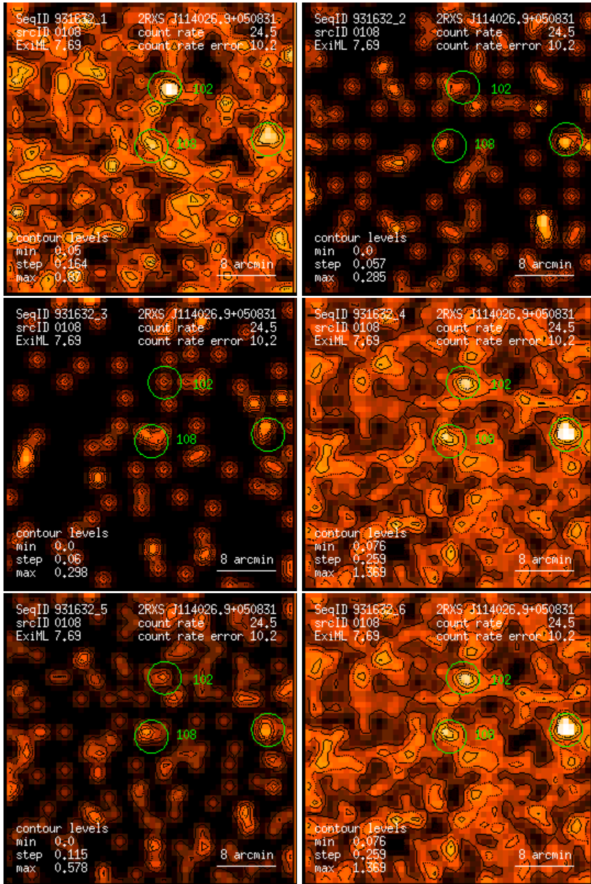
Figure 108: RASS 931632: detection 0108: band rate images, Gaussian filter: (1) PSPC channels 11 – 41, (2) 52 – 90, (3) 91 – 201, (4) 11 – 235, (5) 52 – 201, (6) 11 – 201. Broad band rates in counts/ks. Band rate contour levels in counts/ks/arcmin 2 .
