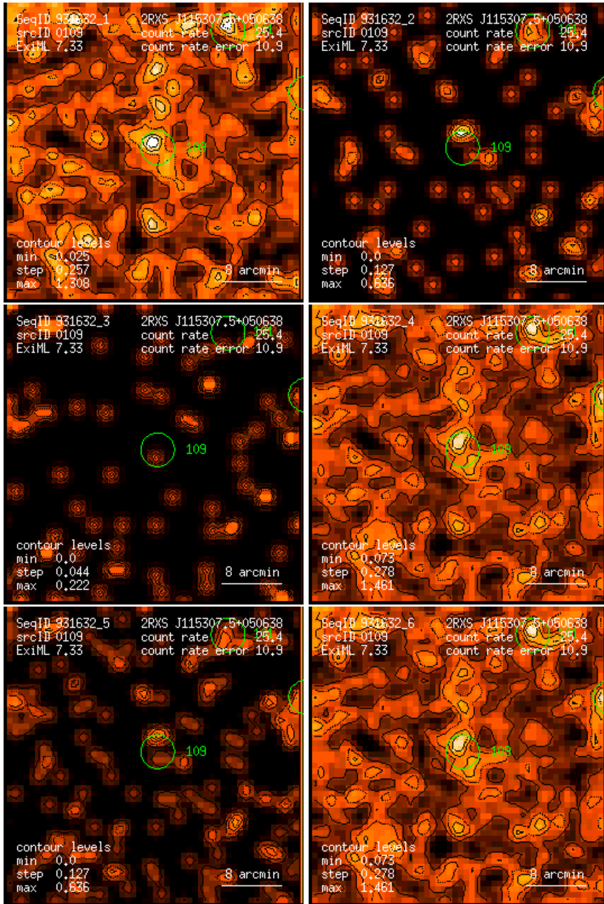
Figure 109: RASS 931632: detection 0109: band rate images, Gaussian filter: (1) PSPC channels 11 – 41, (2) 52 – 90, (3) 91 – 201, (4) 11 – 235, (5) 52 – 201, (6) 11 – 201. Broad band rates in counts/ks. Band rate contour levels in counts/ks/arcmin 2 .
