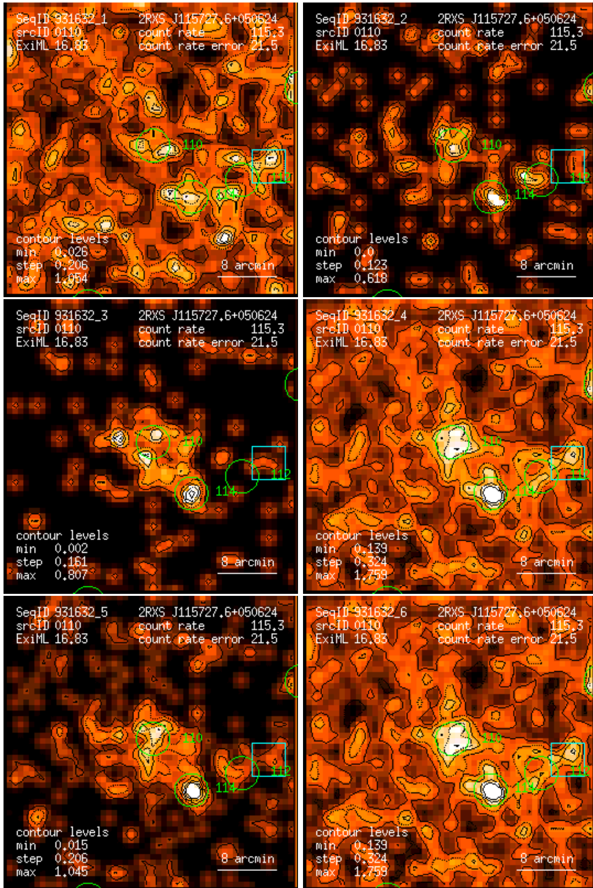
Figure 110: RASS 931632: detection 0110: band rate images, Gaussian filter: (1) PSPC channels 11 – 41, (2) 52 – 90, (3) 91 – 201, (4) 11 – 235, (5) 52 – 201, (6) 11 – 201. Broad band rates in counts/ks. Band rate contour levels in counts/ks/arcmin 2 .
