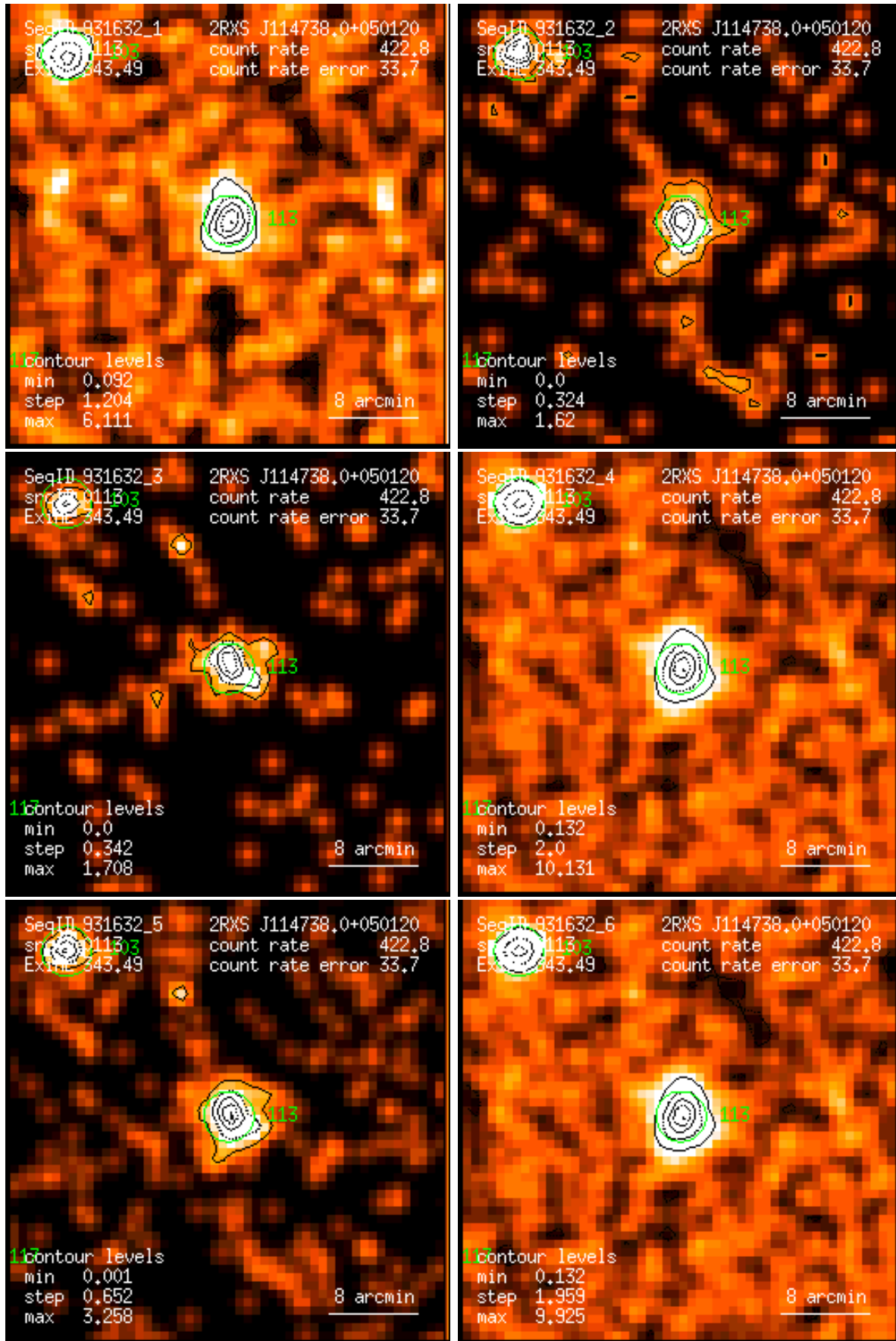
Figure 113: RASS 931632: detection 0113: band rate images, Gaussian filter: (1) PSPC channels 11 – 41, (2) 52 – 90, (3) 91 – 201, (4) 11 – 235, (5) 52 – 201, (6) 11 – 201. Broad band rates in counts/ks. Band rate contour levels in counts/ks/arcmin 2 .
