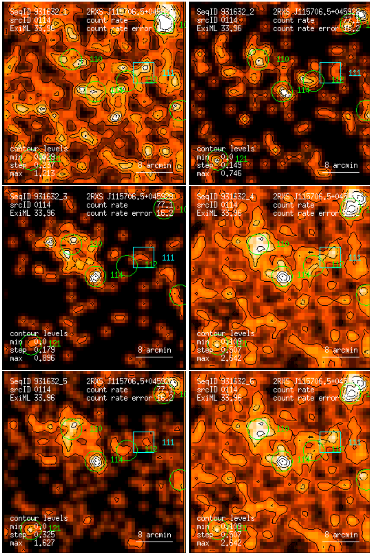
Figure 114: RASS 931632: detection 0114: band rate images, Gaussian filter: (1) PSPC channels 11 – 41, (2) 52 – 90, (3) 91 – 201, (4) 11 – 235, (5) 52 – 201, (6) 11 – 201. Broad band rates in counts/ks. Band rate contour levels in counts/ks/arcmin 2 .
