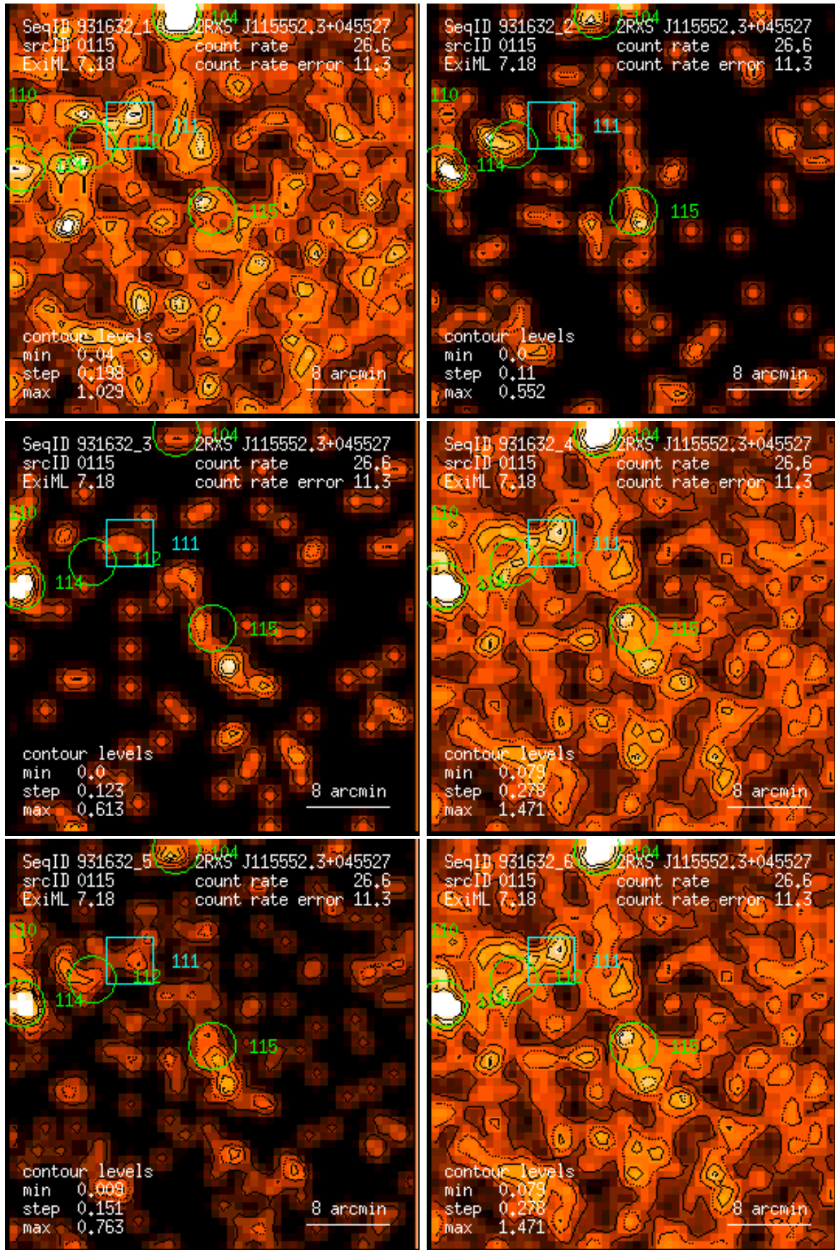
Figure 115: RASS 931632: detection 0115: band rate images, Gaussian filter: (1) PSPC channels 11 – 41, (2) 52 – 90, (3) 91 – 201, (4) 11 – 235, (5) 52 – 201, (6) 11 – 201. Broad band rates in counts/ks. Band rate contour levels in counts/ks/arcmin 2 .
