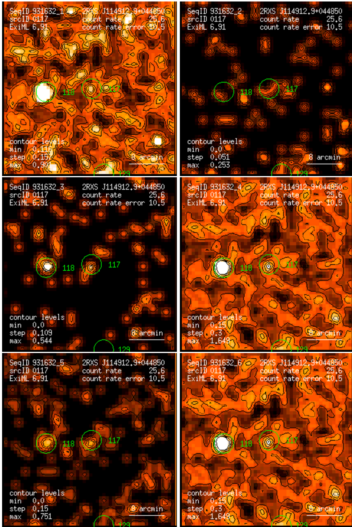
Figure 117: RASS 931632: detection 0117: band rate images, Gaussian filter: (1) PSPC channels 11 – 41, (2) 52 – 90, (3) 91 – 201, (4) 11 – 235, (5) 52 – 201, (6) 11 – 201. Broad band rates in counts/ks. Band rate contour levels in counts/ks/arcmin 2 .
