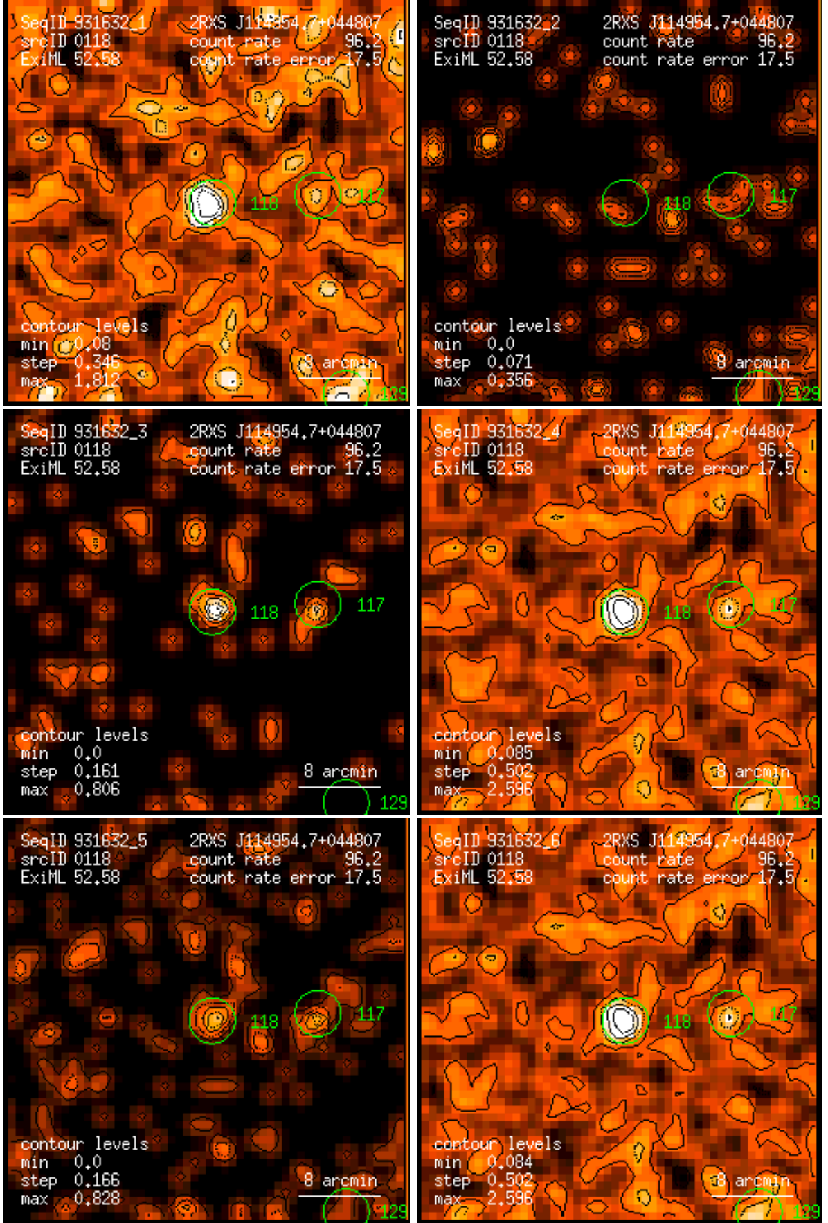
Figure 118: RASS 931632: detection 0118: band rate images, Gaussian filter: (1) PSPC channels 11 – 41, (2) 52 – 90, (3) 91 – 201, (4) 11 – 235, (5) 52 – 201, (6) 11 – 201. Broad band rates in counts/ks. Band rate contour levels in counts/ks/arcmin 2 .
