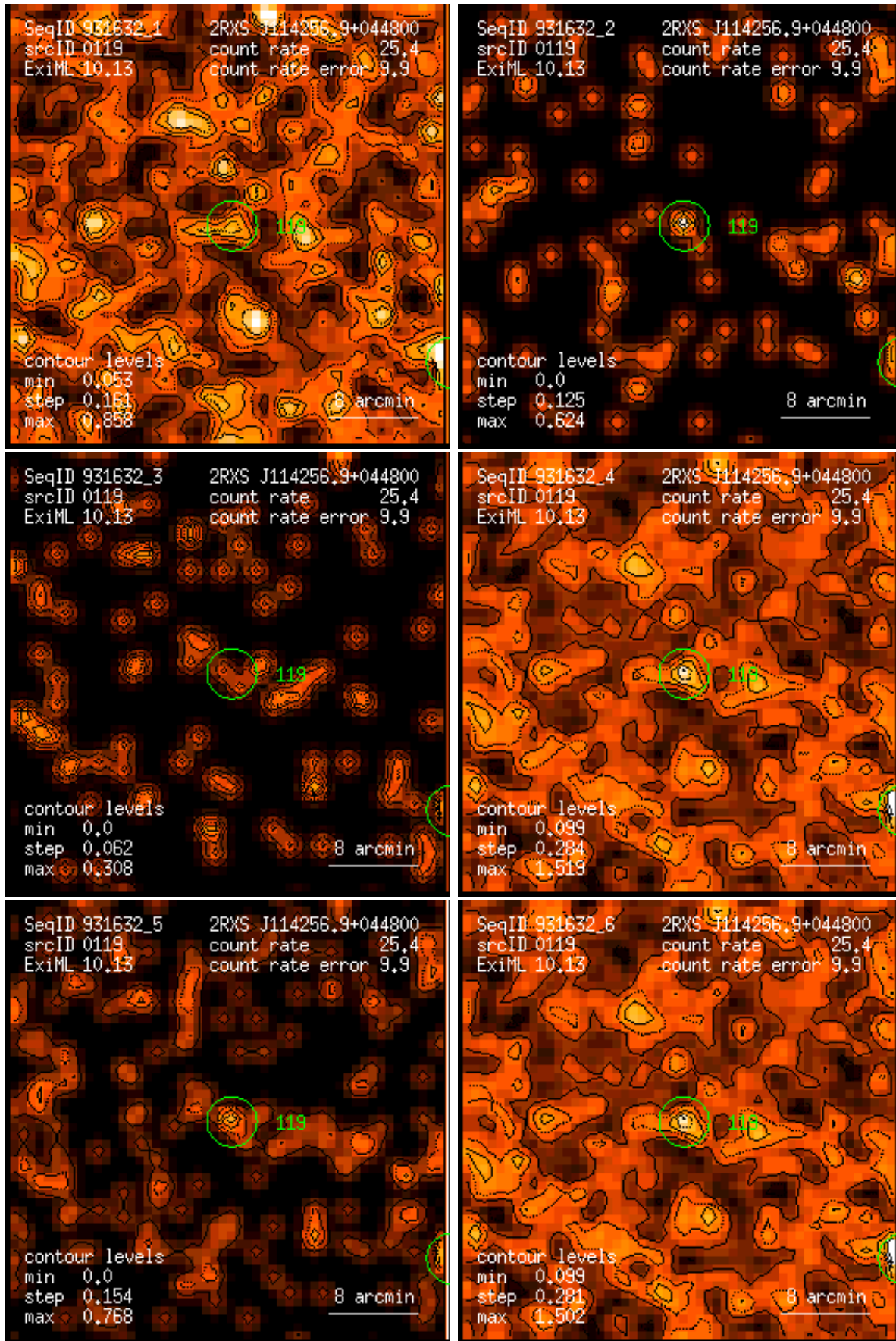
Figure 119: RASS 931632: detection 0119: band rate images, Gaussian filter: (1) PSPC channels 11 – 41, (2) 52 – 90, (3) 91 – 201, (4) 11 – 235, (5) 52 – 201, (6) 11 – 201. Broad band rates in counts/ks. Band rate contour levels in counts/ks/arcmin 2 .
