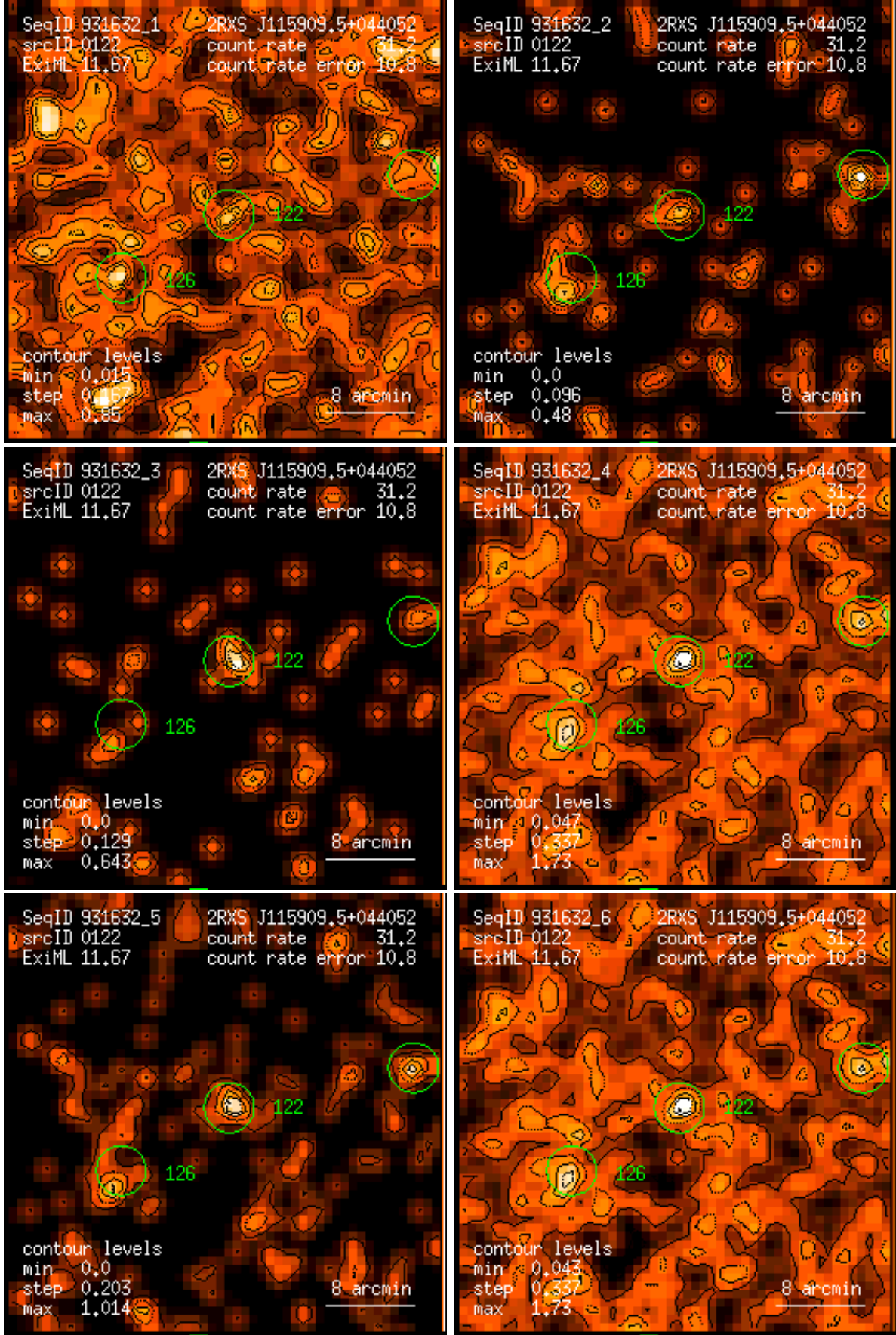
Figure 122: RASS 931632: detection 0122: band rate images, Gaussian filter: (1) PSPC channels 11 – 41, (2) 52 – 90, (3) 91 – 201, (4) 11 – 235, (5) 52 – 201, (6) 11 – 201. Broad band rates in counts/ks. Band rate contour levels in counts/ks/arcmin 2 .
