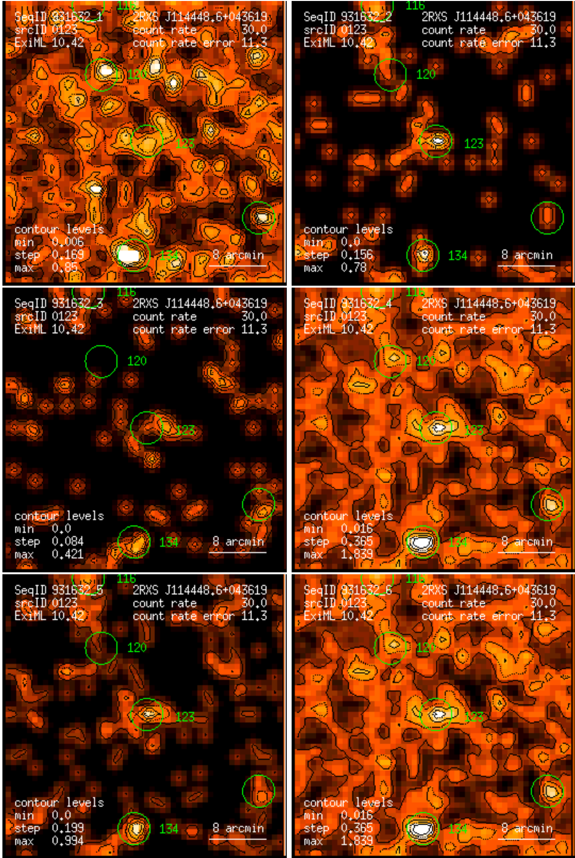
Figure 123: RASS 931632: detection 0123: band rate images, Gaussian filter: (1) PSPC channels 11 – 41, (2) 52 – 90, (3) 91 – 201, (4) 11 – 235, (5) 52 – 201, (6) 11 – 201. Broad band rates in counts/ks. Band rate contour levels in counts/ks/arcmin 2 .
