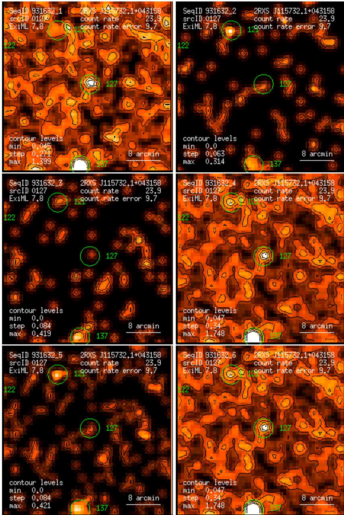
Figure 127: RASS 931632: detection 0127: band rate images, Gaussian filter: (1) PSPC channels 11 – 41, (2) 52 – 90, (3) 91 – 201, (4) 11 – 235, (5) 52 – 201, (6) 11 – 201. Broad band rates in counts/ks. Band rate contour levels in counts/ks/arcmin 2 .
