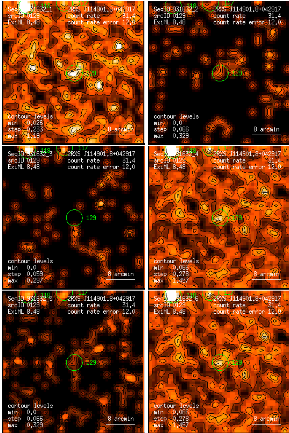
Figure 129: RASS 931632: detection 0129: band rate images, Gaussian filter: (1) PSPC channels 11 – 41, (2) 52 – 90, (3) 91 – 201, (4) 11 – 235, (5) 52 – 201, (6) 11 – 201. Broad band rates in counts/ks. Band rate contour levels in counts/ks/arcmin 2 .
