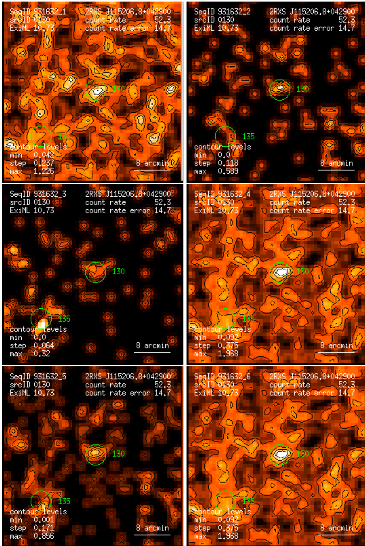
Figure 130: RASS 931632: detection 0130: band rate images, Gaussian filter: (1) PSPC channels 11 – 41, (2) 52 – 90, (3) 91 – 201, (4) 11 – 235, (5) 52 – 201, (6) 11 – 201. Broad band rates in counts/ks. Band rate contour levels in counts/ks/arcmin 2 .
