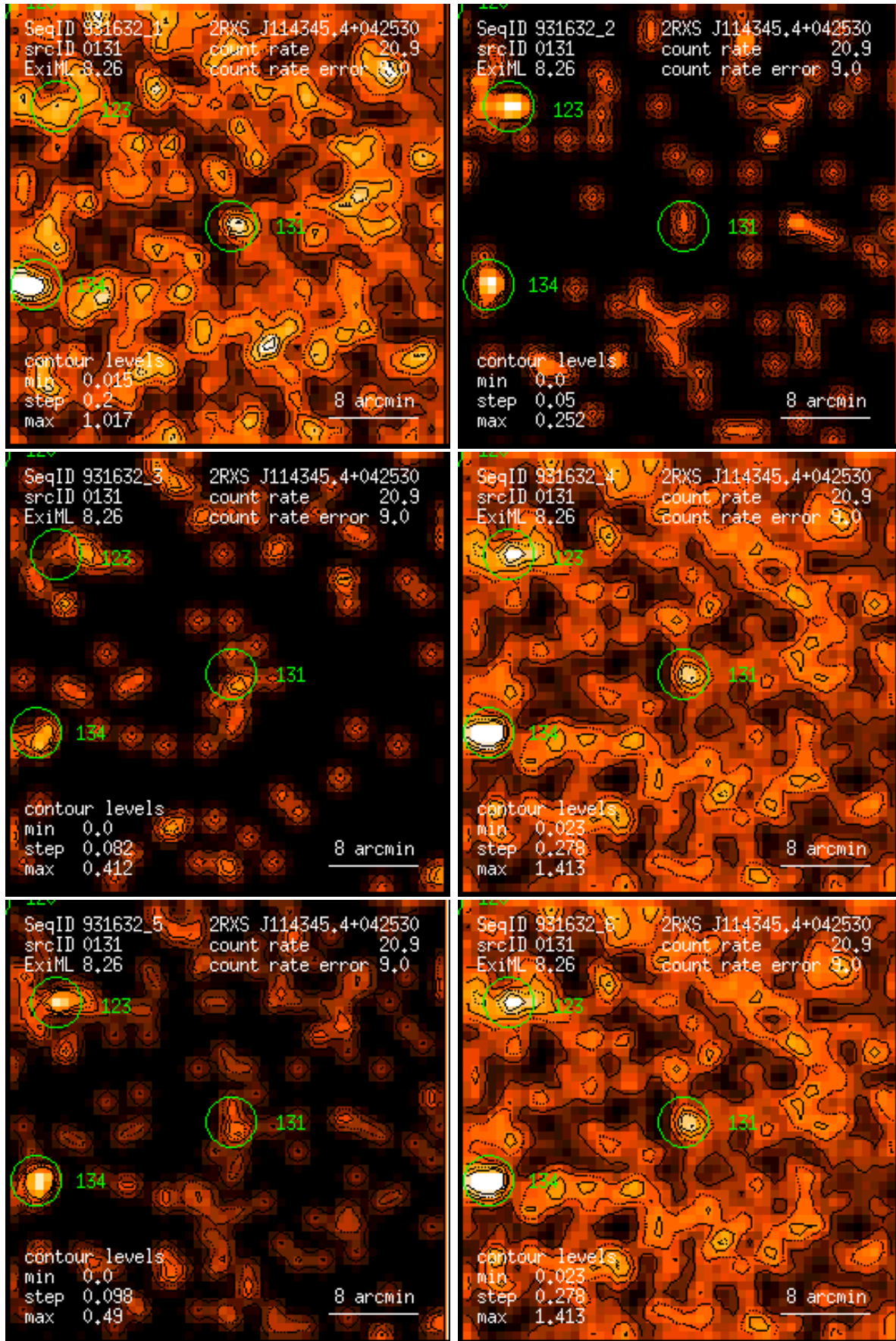
Figure 131: RASS 931632: detection 0131: band rate images, Gaussian filter: (1) PSPC channels 11 – 41, (2) 52 – 90, (3) 91 – 201, (4) 11 – 235, (5) 52 – 201, (6) 11 – 201. Broad band rates in counts/ks. Band rate contour levels in counts/ks/arcmin 2 .
