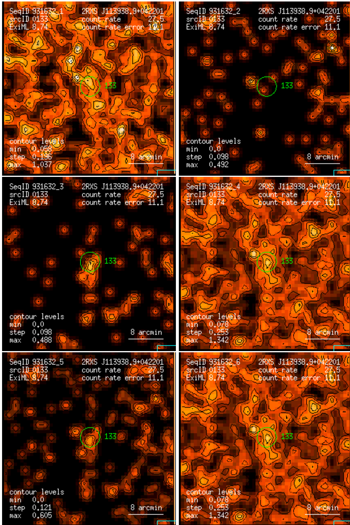
Figure 133: RASS 931632: detection 0133: band rate images, Gaussian filter: (1) PSPC channels 11 – 41, (2) 52 – 90, (3) 91 – 201, (4) 11 – 235, (5) 52 – 201, (6) 11 – 201. Broad band rates in counts/ks. Band rate contour levels in counts/ks/arcmin 2 .
