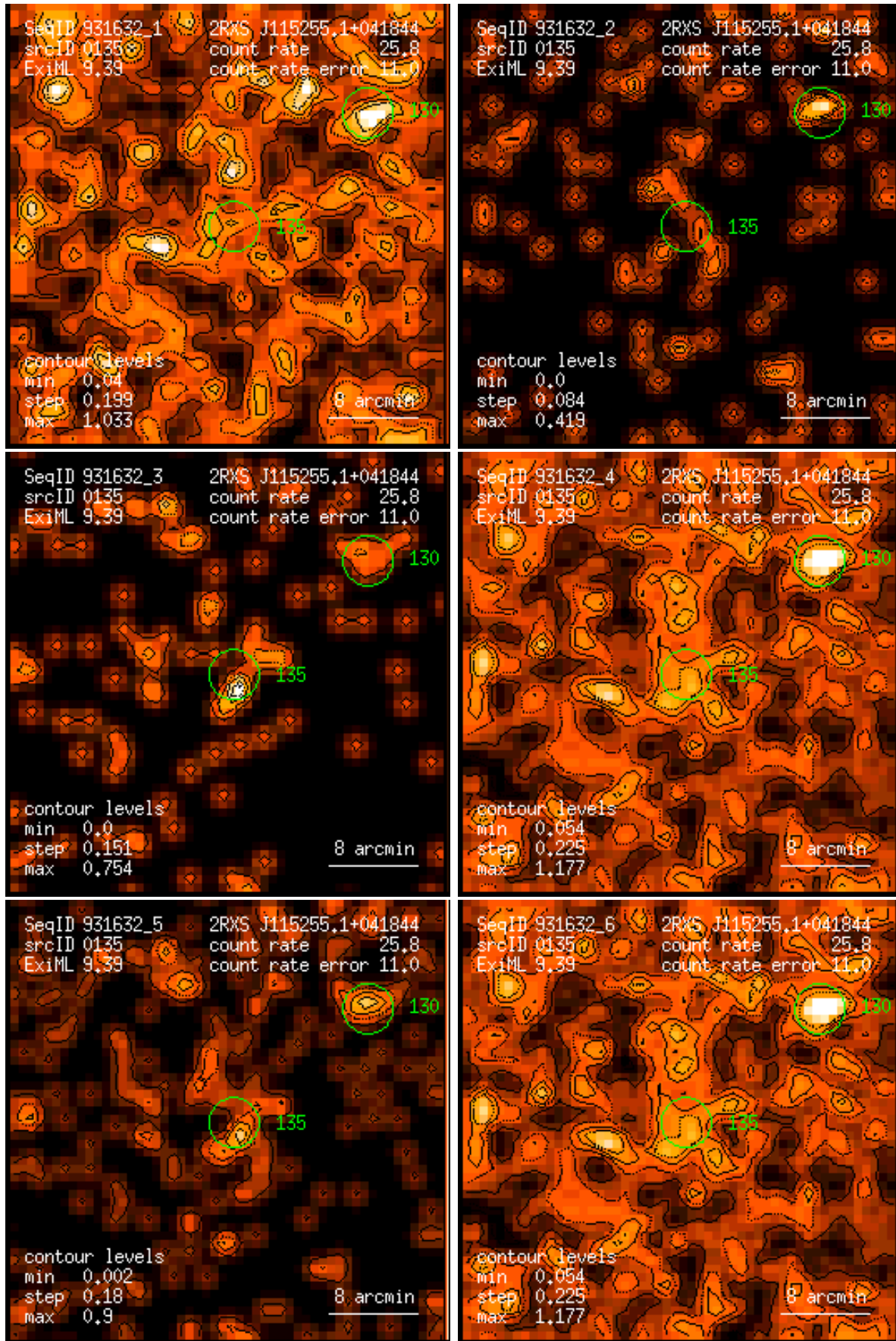
Figure 135: RASS 931632: detection 0135: band rate images, Gaussian filter: (1) PSPC channels 11 – 41, (2) 52 – 90, (3) 91 – 201, (4) 11 – 235, (5) 52 – 201, (6) 11 – 201. Broad band rates in counts/ks. Band rate contour levels in counts/ks/arcmin 2 .
